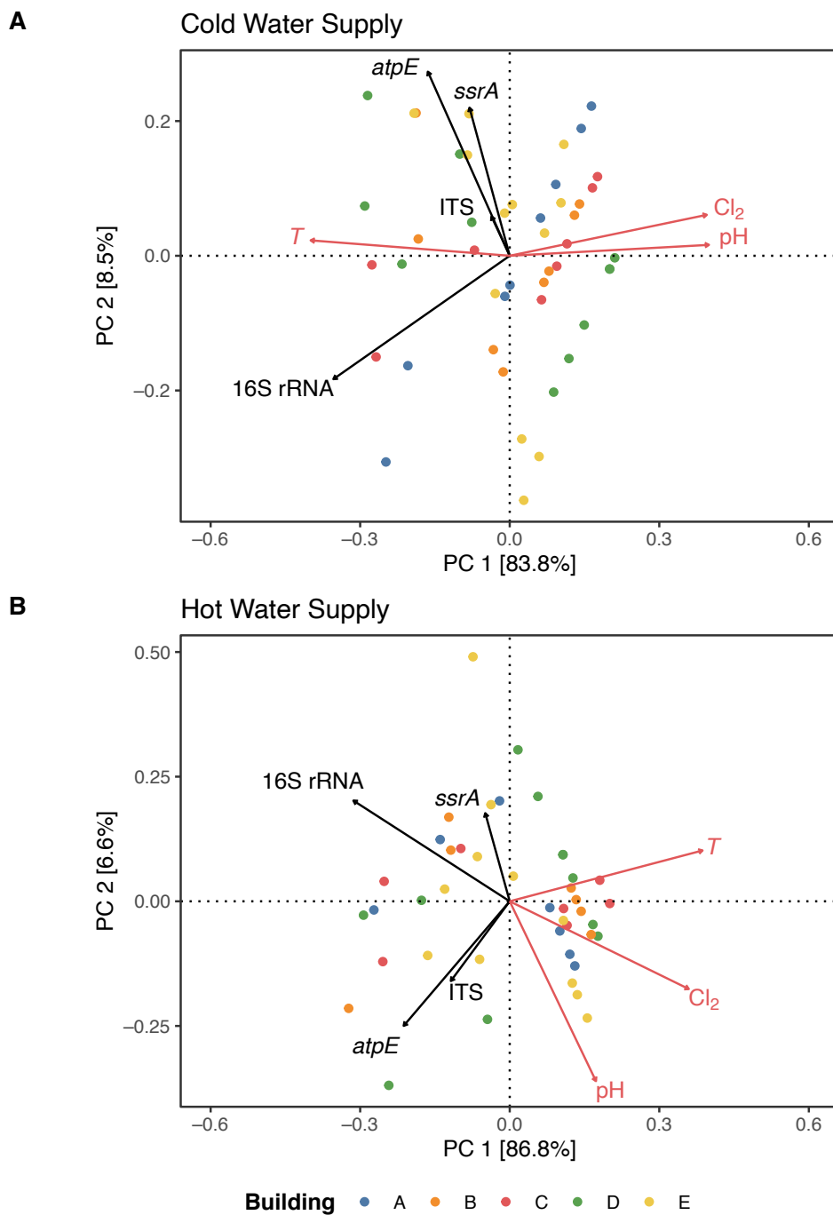
Figure S3. PCA biplot of ranked marker gene concentrations (conditioned by city and building site), with supplemental fitting of water quality parameters (temperature, T ; total chlorine, Cl_2 ; and pH) in (A) cold water supplies, including building inlets, and (B) hot water supplies. Angles between response lines and supplementary variables represent two-dimensional approximations of correlation.
