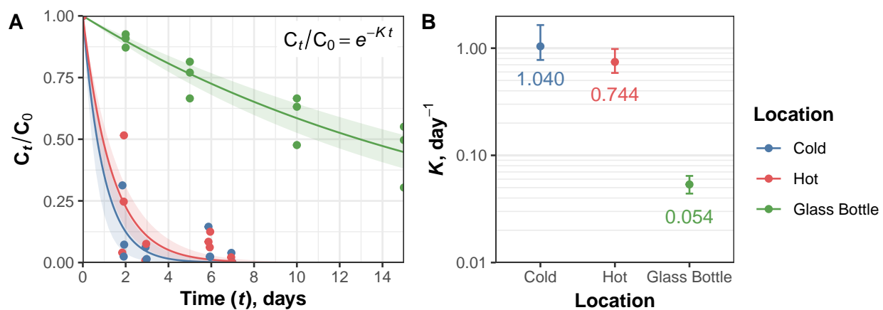
Figure S2. Chloramine decay in Minneapolis cold and hot tap water (onsite observations from buildings A to D) and Minneapolis cold tap water in a laboratory glass bottle: (A) Exponential modelling of chloramine decay as a function of time after flushing ( C_t , relative to initial concentration, C_0 ), with 95% confidence intervals, and (B) the fitted decay rate constants ( K ) with 95% confidence intervals.
