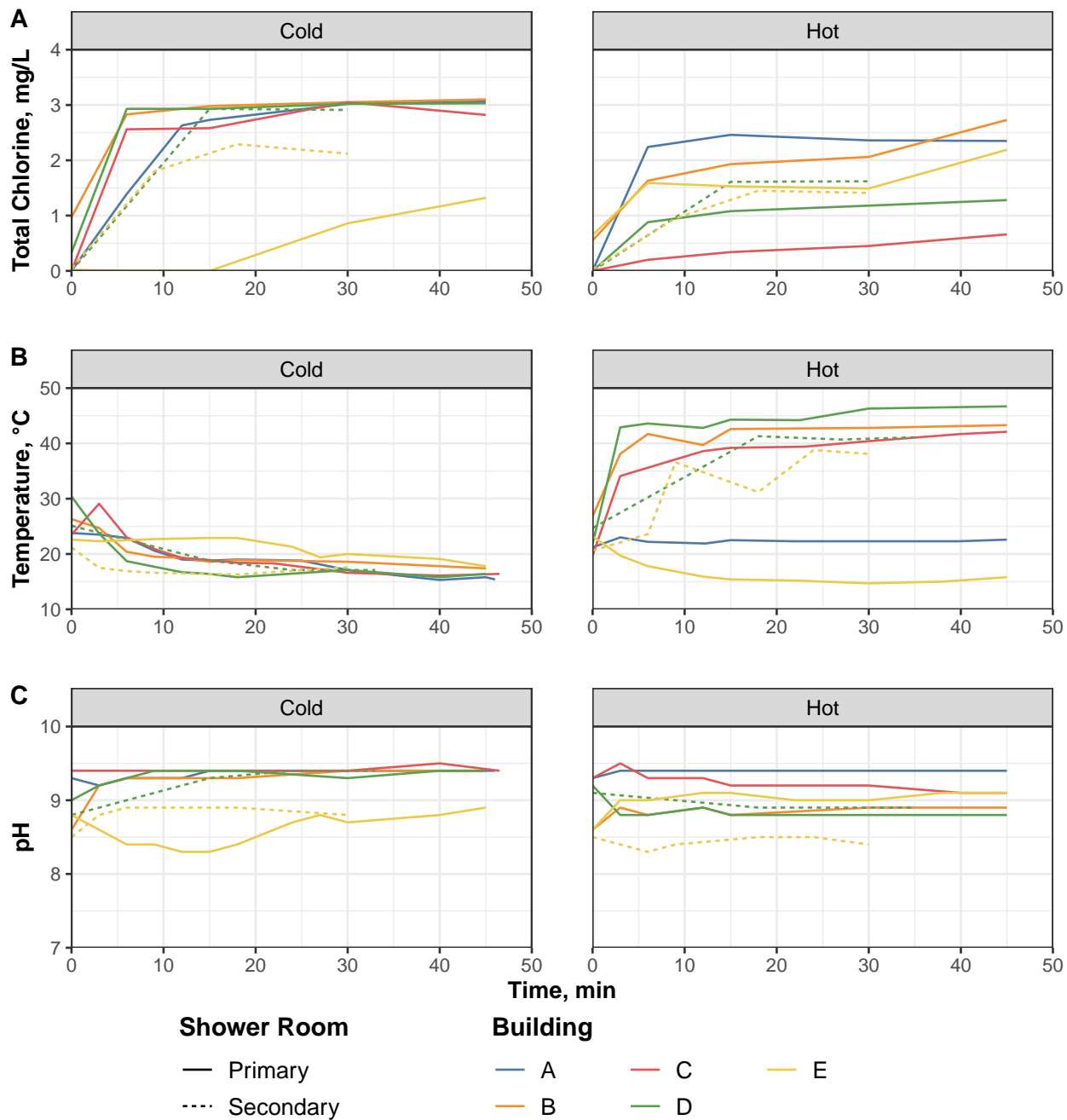
Figure S1. Water quality during flushing: (A) total chlorine, (B) water temperature, and (C) water pH.
