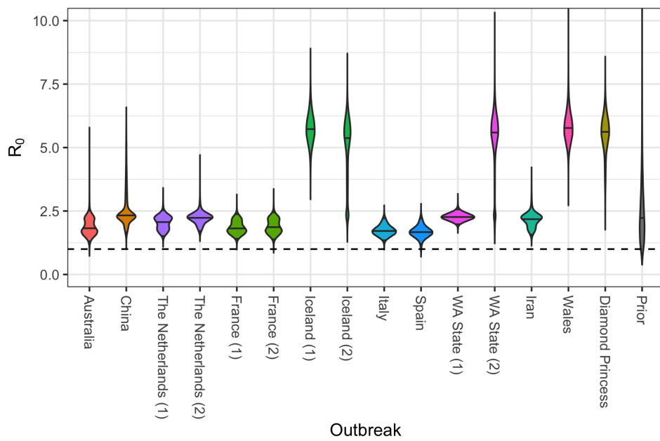
Figure S2: Comparison of R_0 posterior distributions estimated using Bayesian model averaging. (Only the value prior to the quarantine aboard the Diamond Princess was included in this averaging.)
