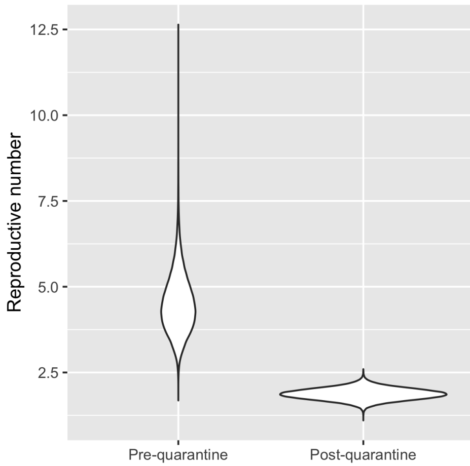
Figure S3: Comparison of R_0 posterior distributions estimated for the pre- and post-quarantine phases of the Diamond Princess outbreak.
