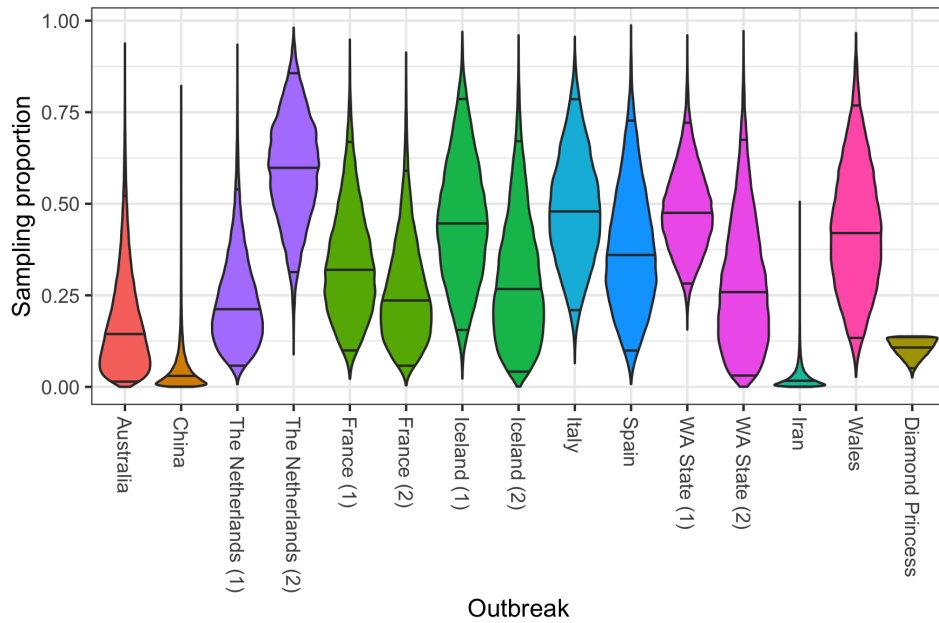
Figure S4: Inferred sampling proportions corresponding to the outbreaks analyzed. Non-informative priors were used for all sampling proportions except for the one corresponding to the Diamond Princess. (See methods).
