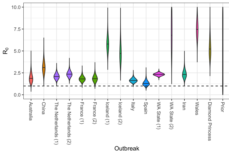
Figure S9: Estimates of R_0 produced using the alternative prior \text{Unif}(0, 10) , illustrating the insensitivity of the results to the precise prior used.
