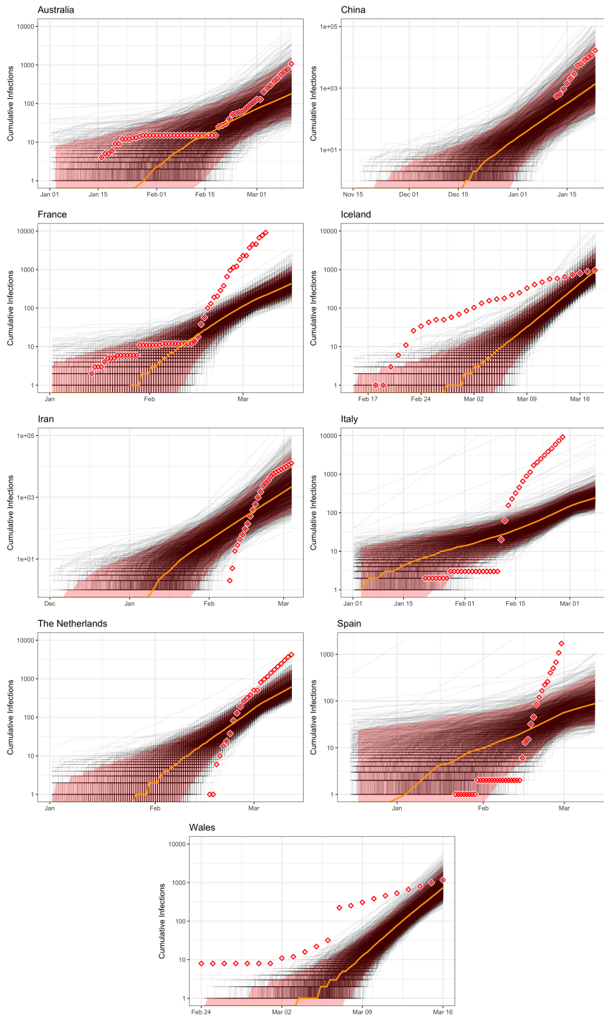
Figure S6: Inferred cumulative case trajectories for remaining outbreaks.
