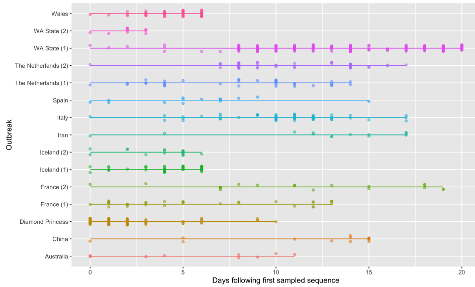
Figure S7: Sample times relative to first sample from each outbreak. Horizontal bars represent full sample period lengths.
