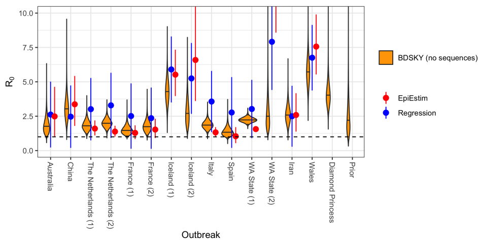
Figure S5: R_0 values inferred using (a) phylodynamic method without sequence data, (b) EpiEstim (1) analysis of sequenced sample collection times, and (c) linear regression of outbreak-specific cumulative sample count distributions. (The Diamond Princess regression and EpiEstim results have been excluded from this graphic, as they relate to the post- rather than pre-quarantine phase of that outbreak.)
