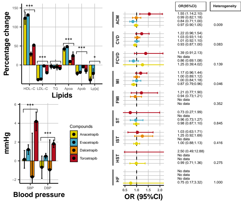
Figure S1: Random effects meta-analyses of CETP inhibitors. The difference column presents a p-value for the difference in OR across the 4 compounds. Similarly, *** heterogeneity p-value < 0.001, ** 0.01 < p-value < 0.001, * 0.05 < p-value < 0.01, . p-value < 0.05. Abbreviations: LDL-C, low-density lipoprotein cholesterol; HDL-C, high-density lipoprotein cholesterol; TG, triglycerides; ApoB, apolipoprotein B; ApoA1, apolipoprotein A1; Lp[a], lipoprotein[a]; SBP, systolic blood pressure; DBP, diastolic blood pressure; ACM, all-cause mortality; CVD, any cardiovascular disease; FCVD, fata-CVD; MI, any myocardial infarction; FMI, fatal-MI; ST, stroke; IST, ischemic ST; HST, hemorrhagic ST; HF, heart failure.
