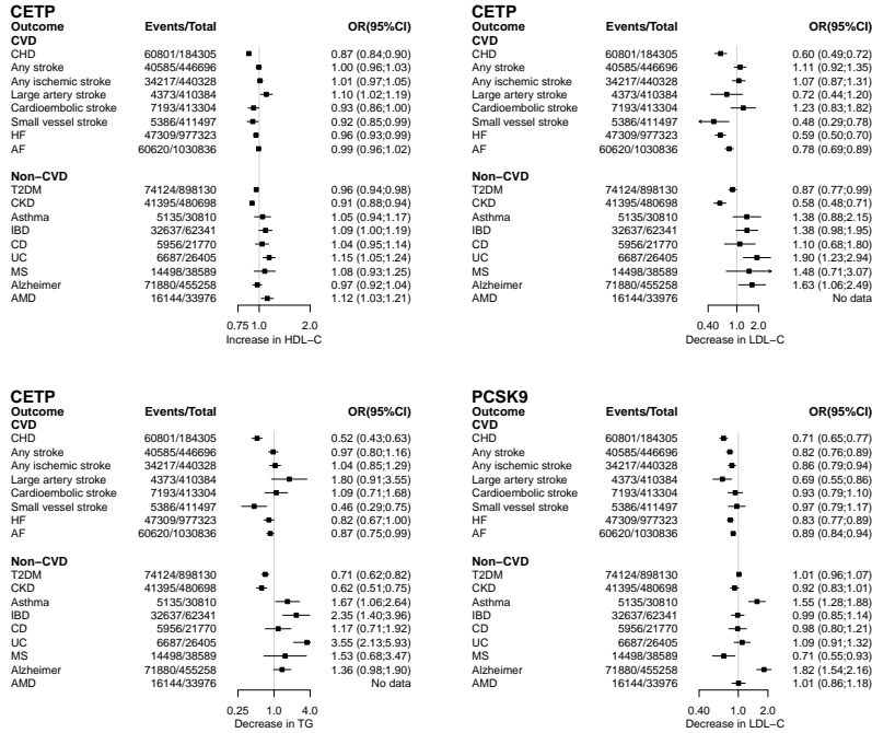
Figure S2: Drug target MR effects of CETP and PCSK9 clinically relevant outcomes proxied by the genetic effects on LDL-C (for CETP and PCSK9 ), HDL-C and TG (for CETP ). Results are coded in the canonical, treatment direction (HDL-C increase, LDL-C and TG decrease).
