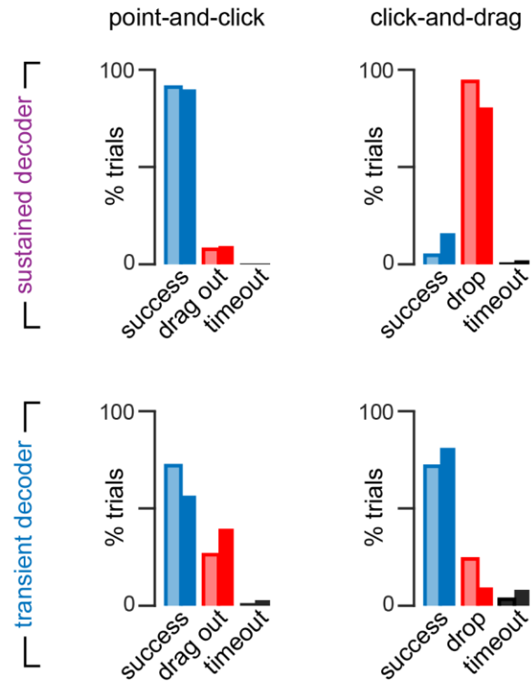
Figure S1 Outcome distributions for all conditions if early clicks are allowed.
