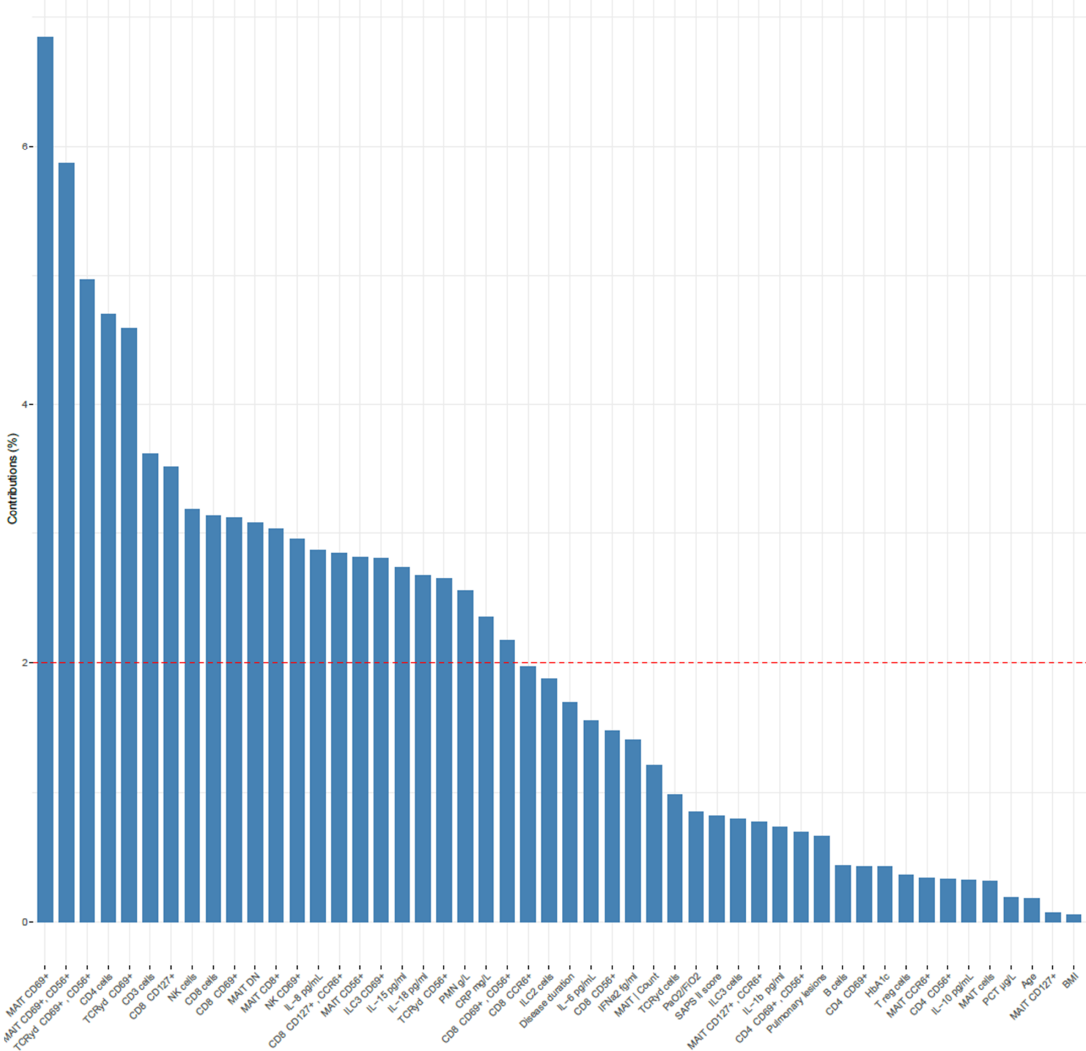
Supplementary Fig. 9: All contribution parameters in Principal Component Analysis (PCA) of all COVID-19 patients. Contribution variables used to produce the PCA including non-fatal cases of IDU (n=46), ICU (n=30), and fatal cases from IDU (n=6) and ICU (n=21) SARS-CoV-2 infected patients. Dotted line symbolizes if all variable contributions were identical.
