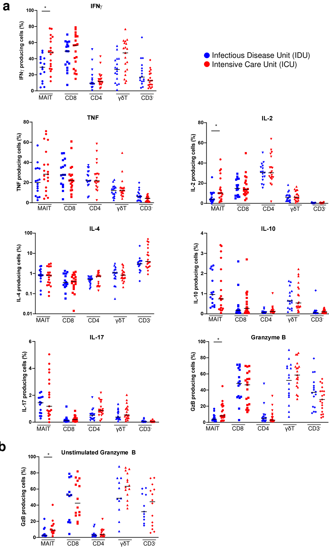
Supplementary Fig. 5: MAIT cell function alterations scale with COVID-19 severity. (a) Flow cytometry analysis of IFN \gamma , TNF, IL-2, IL-4, IL-10, IL-17 cytokine, and granzyme B production among stimulated MAIT cells, conventional CD8 + and CD4 + T cells, \gamma\delta T and CD3 - cells from IDU (n=15-16) or ICU COVID-19 patients (n=19). (b) Flow cytometry analysis of GzB without stimulation from IDU (n=11) or ICU COVID-19 patients (n=14). Each symbol represents a single biological sample. *P<0.05 and **P<0.01 (two-sided Mann-Whitney nonparametric test).
