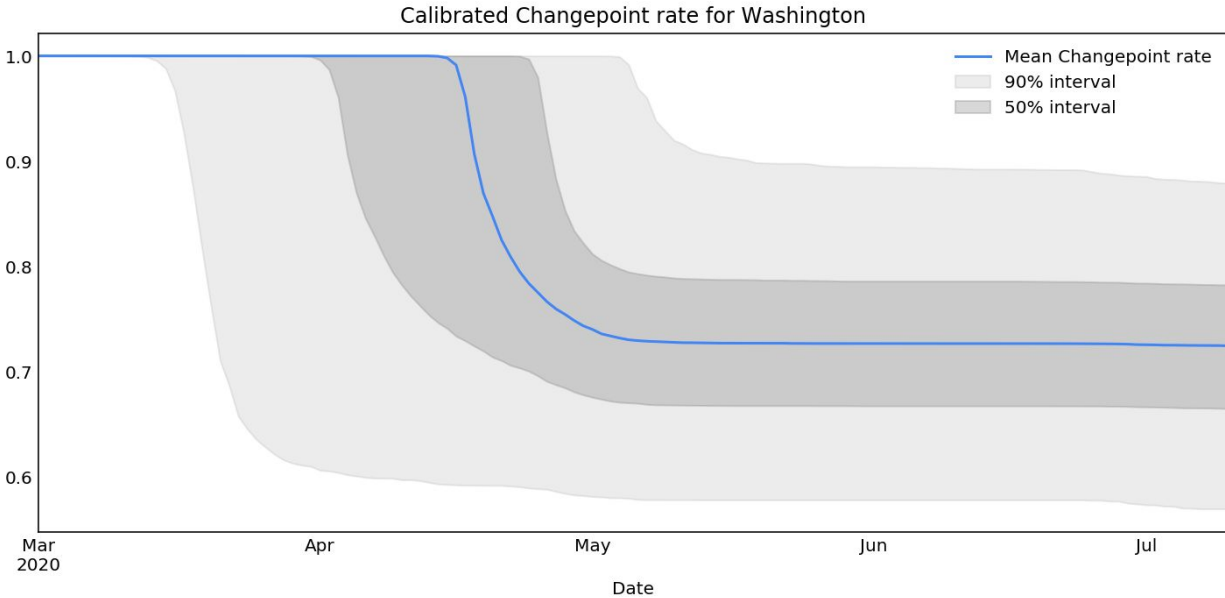
Fig. S3. The coefficients of a latent changepoint, modeled as a negative sigmoid, fit as part of the Bayesian SEIR model to predict the time-varying infection rate. The learned coefficients are used to scale the time-dependent infectious rate in the OpenABM-Covid19 model.
