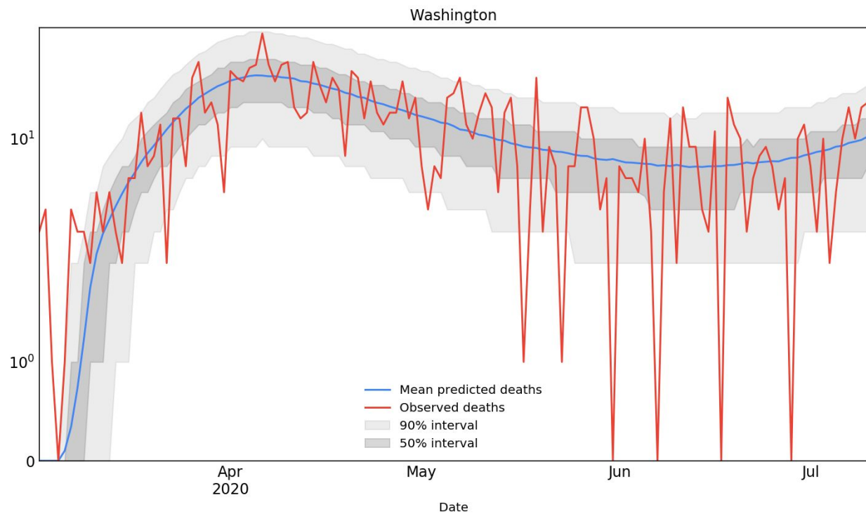
Fig. S1. A Bayesian SEIR model fit to Washington state epidemiological data allowing infection rate to vary as a function of human mobility and a latent changepoint to account for unobserved changes in human behavior. See Liu et al. (36) for more detail on the methodology.
