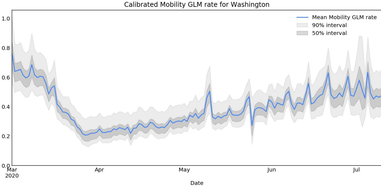
Fig. S2. The coefficients from the a generalizable linear model (GLM) fit as part of the above Bayesian SEIR model to predict the time-varying infection rate as a function of aggregated and anonymized mobility data from the Community Mobility Reports. The learned coefficients are used to scale the number of synthetic agent interactions in the random and occupation networks in the OpenABM-Covid19 model.
