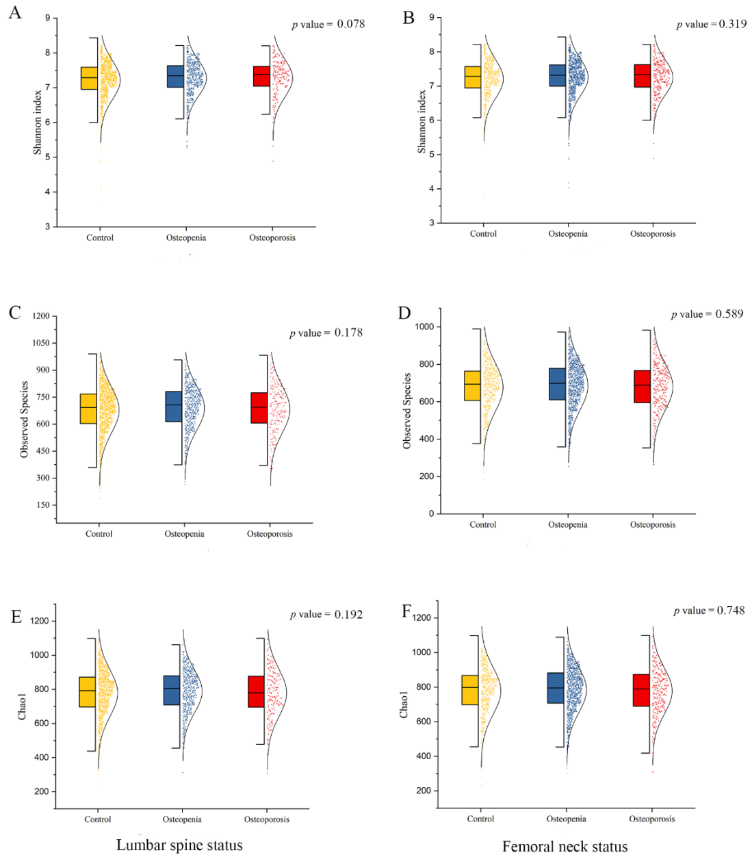
Figure S1. \alpha diversity estimator, measured using the 16S rRNA gene OTUs. A and B, Shannon index within subjects by lumbar spine and femoral neck status. C and D, Observed species within subjects by lumbar spine and femoral neck status. E and F, Chao1 within subjects by lumbar spine and femoral neck status.
