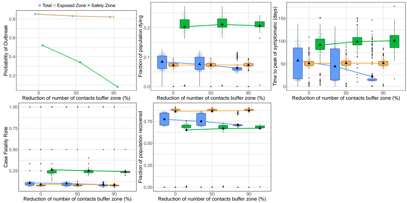
Figure 12: Lockdown of the safety zone. Probability of an outbreak (top left), fraction of the population dying (top middle), time until peak symptomatic cases (top right), CFR (bottom left), and fraction of the population that recovers (bottom middle) as a function of the reduction in the number of contacts permitted in the buffer zone from a baseline of 2 per person in the safety zone per week. All figures consider the scenario in which 20% of the camp's population is allocated to the safety zone.
