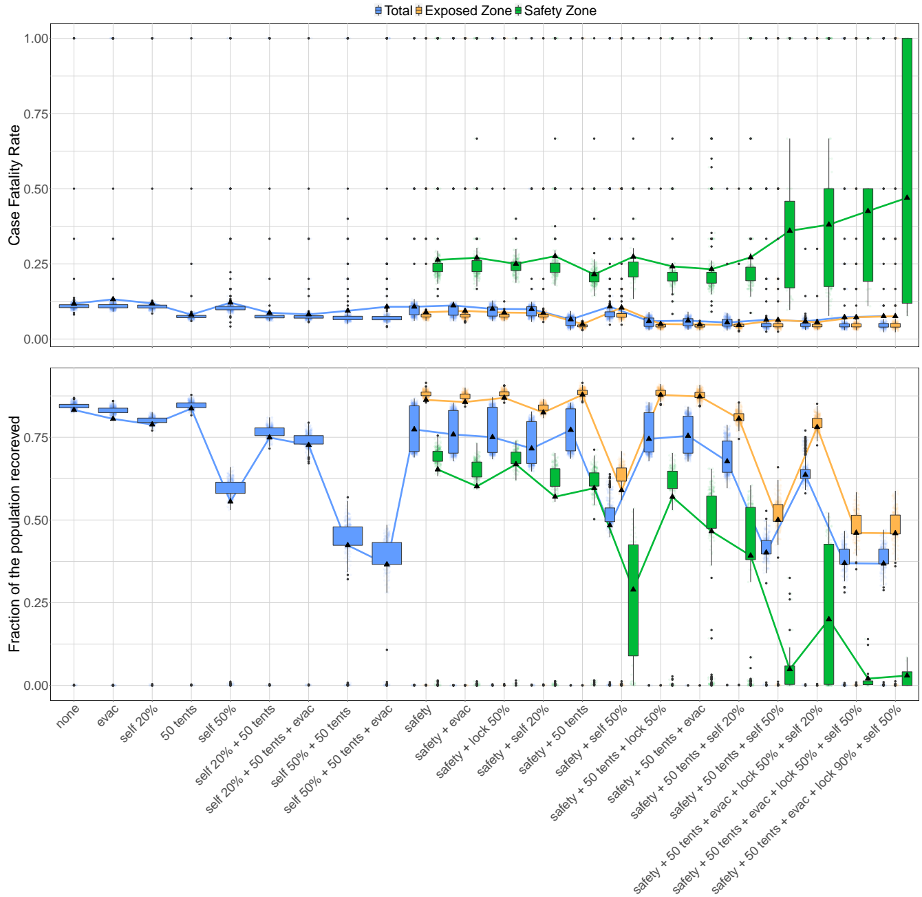
Figure 13: Combined interventions. CFR (top), and fraction of the population that recovers (bottom) for different combinations of interventions. Evac = evacuation of severely symptomatic, self = self-distancing, tents = number of available self-isolation tents, safety = safety zone, lock = lockdown of the buffer zone. For combinations of interventions including a safety zone, we distinguish between the population living in the green zone, in the orange zone and the whole population. The increase in the CFR for the green zone is explained by the discretization of the possible values that the CFR can take when the number of cases is very low (see Supplementary Table 4).
