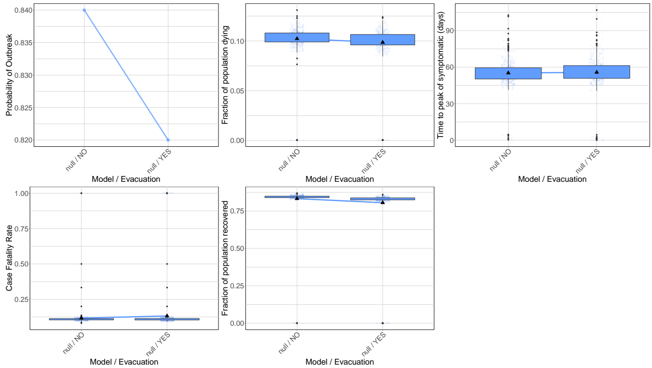
Figure 6: Evacuation. Probability of an outbreak (top left), fraction of the population dying (top middle), time until peak symptomatic cases (top right), CFR (bottom left), and fraction of the population that recovers (bottom middle), as a function of whether individuals requiring hospitalization are evacuated to isolation centers.
