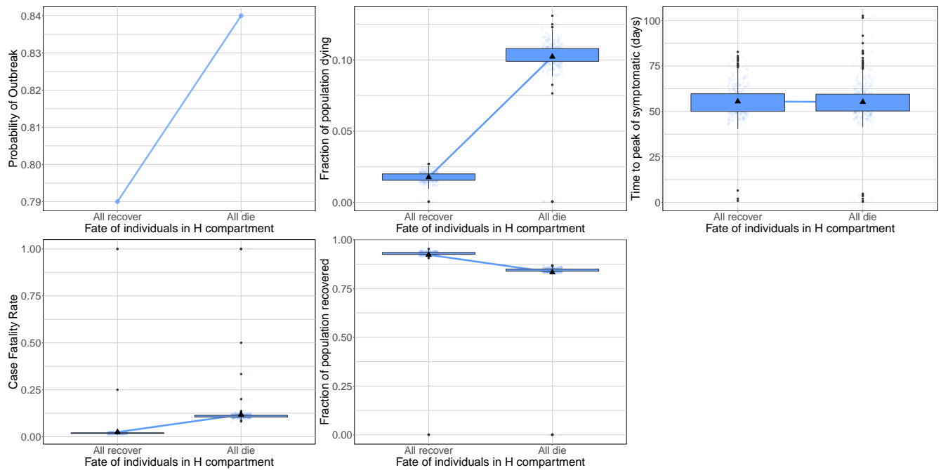
Figure 2: Outcomes when all severe cases recover vs when all severe cases die. Probability of an outbreak (top left), fraction of the population dying (top middle), time until peak symptomatic cases (top right), CFR (bottom left), and fraction of the population that recovers (bottom middle).
