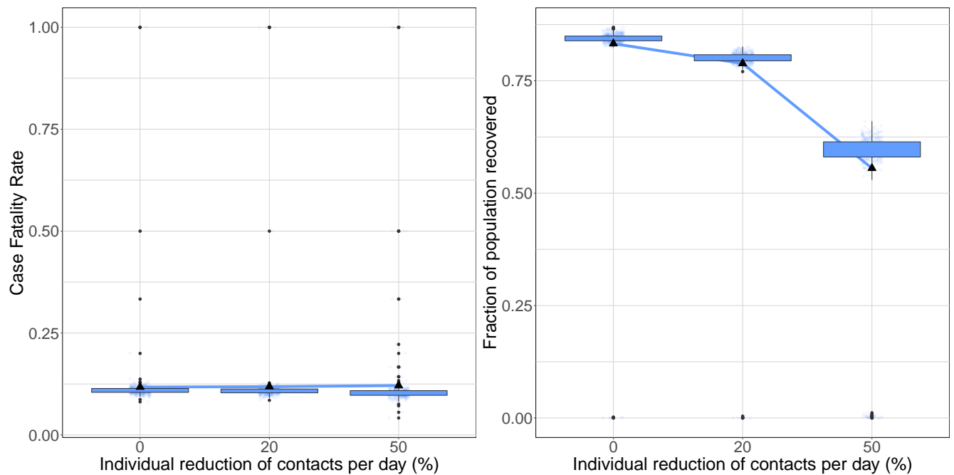
Figure 3: Self-distancing. CFR (left), and fraction of the population that recovers (right) as a function of the proportion of contacts reduced per individual per day.
