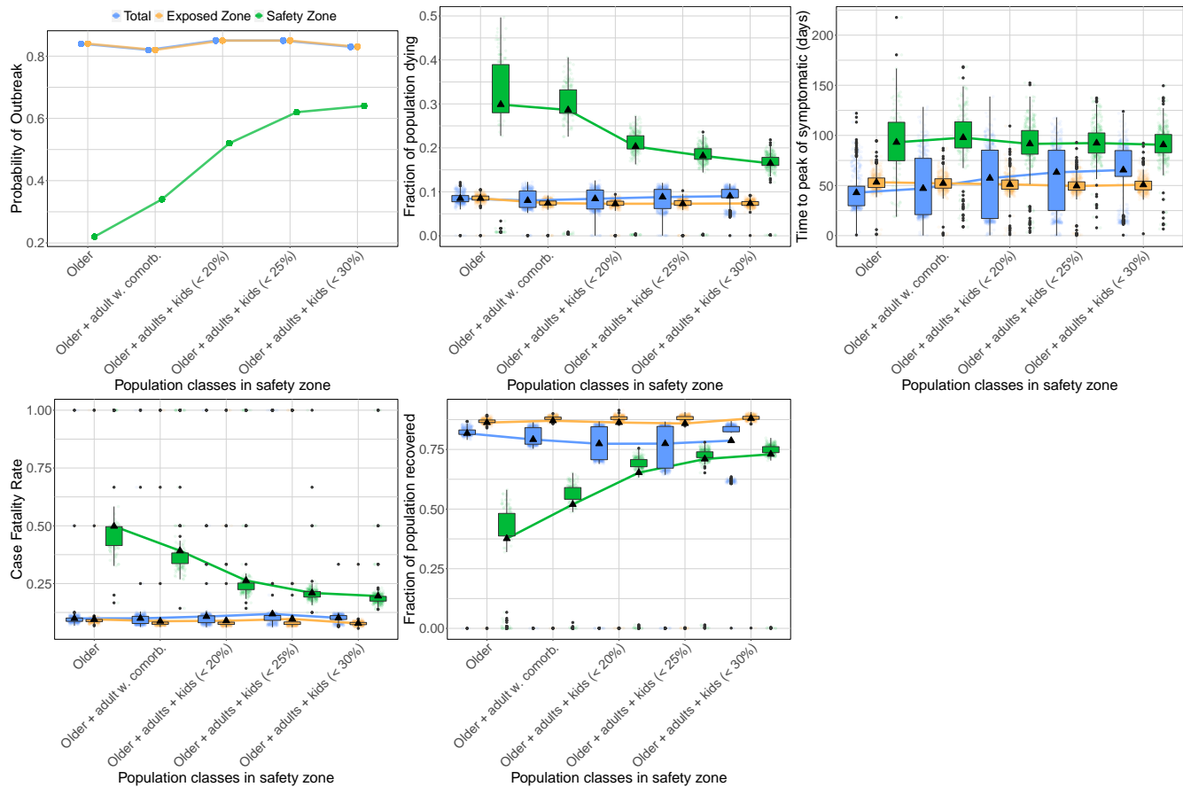
Figure 10: Population moving to the safety zone. Probability of an outbreak (top left), fraction of the population dying (top middle), time until peak symptomatic cases (top right), CFR (bottom left), and fraction of the population that recovers (bottom middle) as a function of the safety zone allocation scenario (see Table 3). All figures consider the scenario with 2 contacts in the buffer per person in the safety zone per week.
