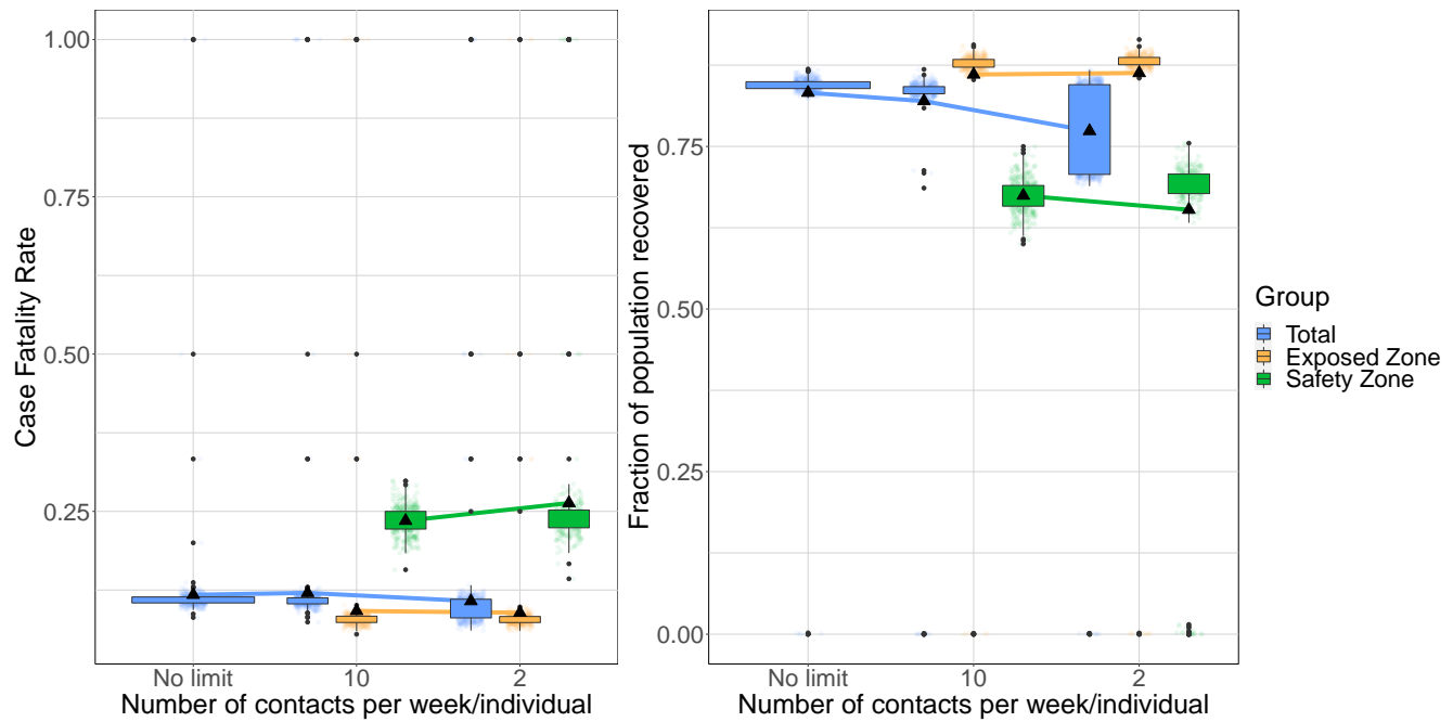
Figure 9: Number of contacts in the buffer zone. CFR (left), and fraction of the population that recovers (right) as a function of the number of contacts that each individual in the safety zone has in the buffer zone per week. All figures consider the scenario in which 20% of the camp's population is allocated to the safety zone.
