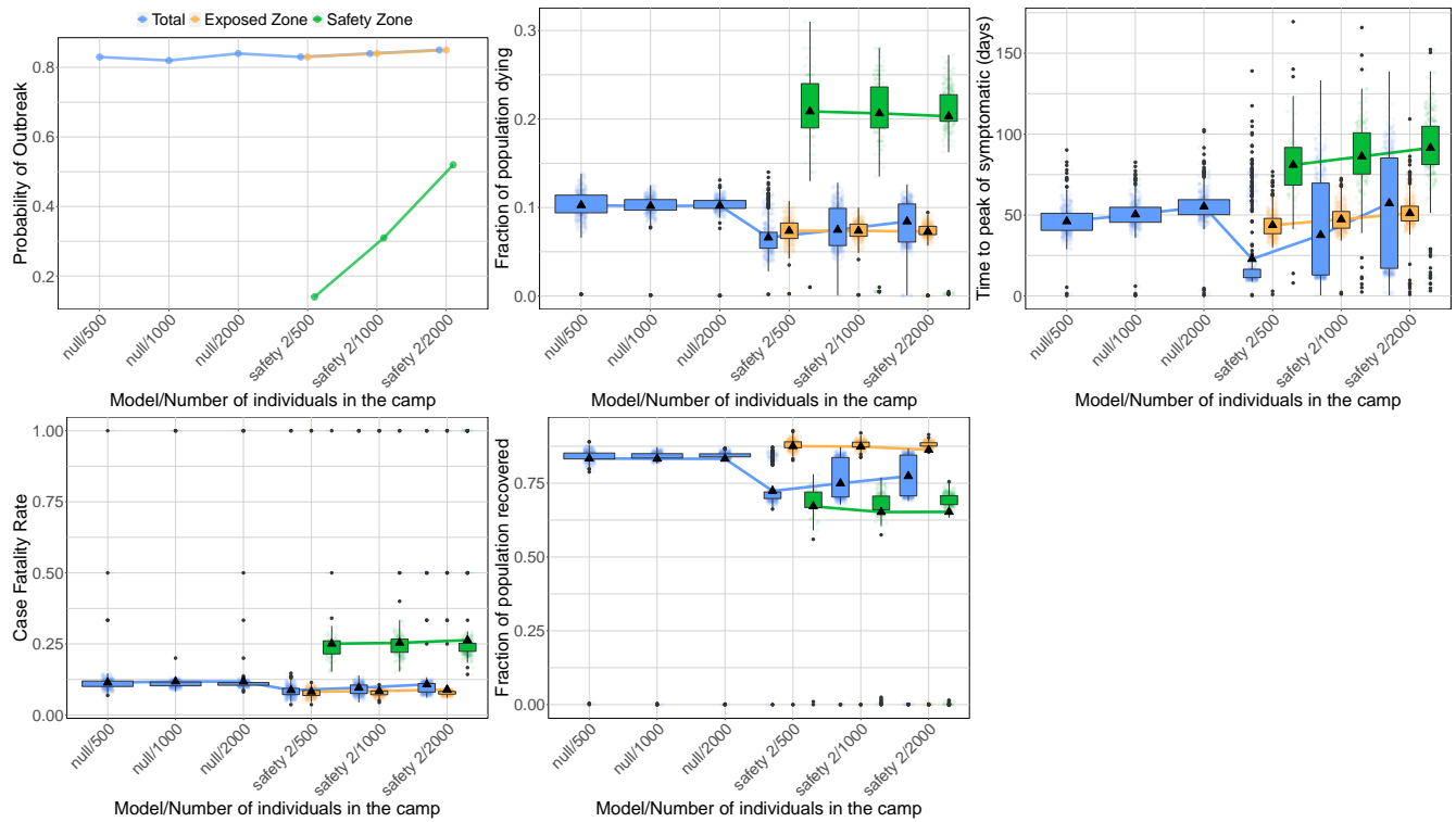
Figure 11: Efficacy of the safety zone for different population sizes. Probability of an outbreak (top left), fraction of the population dying (top middle), time until peak symptomatic cases (top right), CFR (bottom left), and fraction of the population that recovers (bottom middle) as a function of the total population size. The figures consider scenarios with no interventions (null), and with a safety zone comprising 20% of the camp’s population with 2 contacts in the buffer zone per person in the safety zone per week (safety 2).
