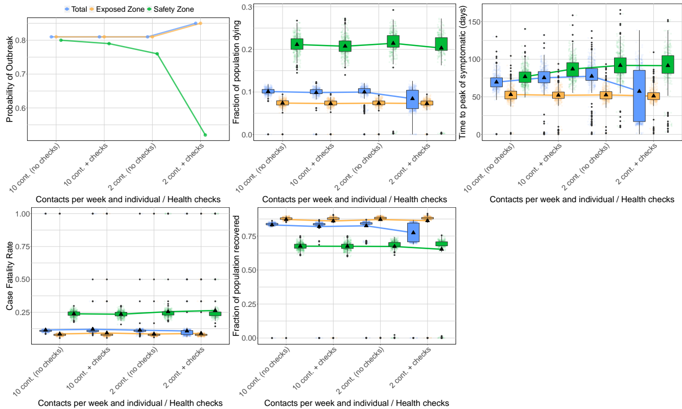
Figure 7: Health-checks in the buffer zone. Probability of an outbreak (top left), fraction of the population dying (top middle), time until peak symptomatic cases (top right), CFR (bottom left), and fraction of the population that recovers (bottom middle), as a function of whether health-checks are implemented in the buffer zone between the safety and exposed zones. Scenarios with 10 or 2 contacts in the buffer zone per person in the safety zone per week are plotted. All figures consider the scenario in which 20% of the camp's population is allocated to the safety zone.
