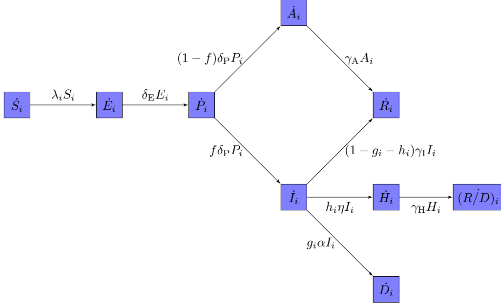
Figure 1: Diagram of the model. The model considers the following compartments: susceptible (S), exposed (E), infectious-presymptomatic (P), infectious-asympomatic (A), infectious-symptomatic (I), infectious-requiring hospitalization (H), recovered (R) and dead (D). Our model considers 3 potential outcomes for symptomatic cases (I): mild cases will recover (R) after the typical infectious period, severe cases will have an extended infectious period during which they require hospitalization (H), and critical cases requiring ICU care will die (D) after the symptomatic period. Since the fate of individuals in the H compartment is uncertain if healthcare is not available, we run simulations considering two possibilities: either all recover, or all die, represented by the R/D compartment.
