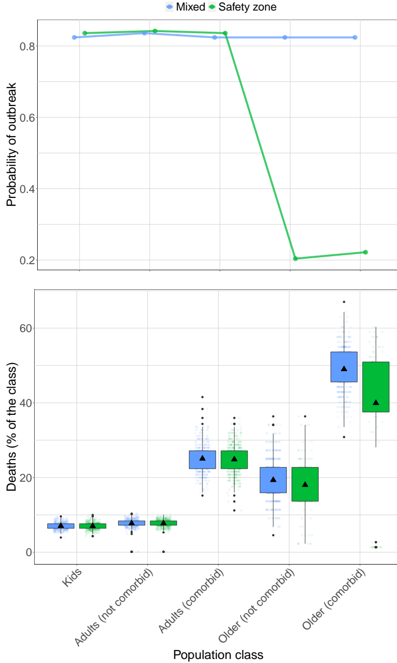
Figure 8: Effects of the safety zone on outcomes by population class. Probability of an outbreak (top), and proportion that dies in each population class (bottom) when no interventions are implemented (Mixed), compared to protection of older adults in the safety zone with 2 contacts in the buffer zone per week (Safety zone). The fraction of deaths in the safety zone for the older population is significantly lower (Kruskal-Wallis test, p\text{-val} < 10^{-15} ).
