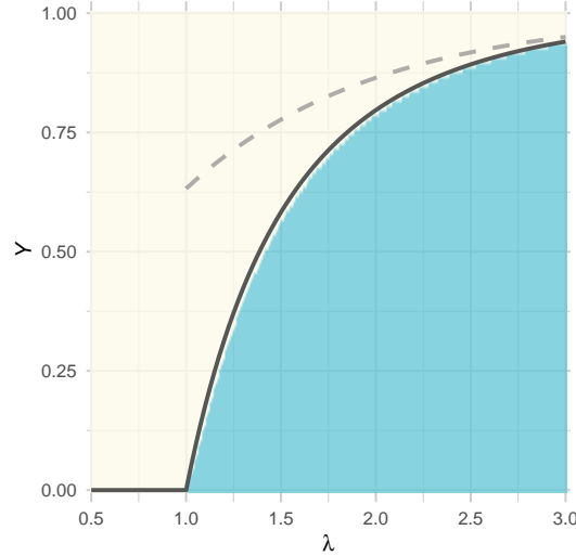
Figure S2. Value of X giving the minimum value of Eq. (S3), as a function of Y and \lambda , based on numerical simulation of the clorSIR model. A clear transition from X = 0 (yellow) to X = 1 (blue) is seen, with no intermediary values. The solid black line corresponds to the theoretical closed-form solution from Eq. (S7), while the dashed grey line corresponds to the rough approximation Y > 1 - e^{-\lambda} past which it is best to not have any closures.
