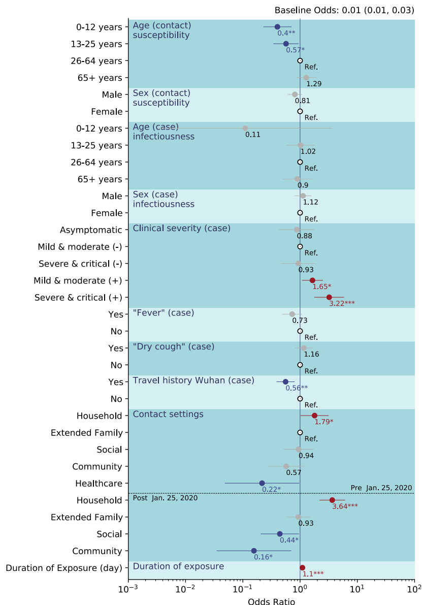
Fig. S8. A sensitivity analysis of GLMM-logit regression that removes missing values. The predictors of the logistic regression as those indicated on the left (fixed effects) and we also include random effects for individual SARS-CoV-2 infections. The “(-)” in “Mild & Moderate (-)” and “Sever & Critical (-)” indicate the SARS-CoV-2 infected individual’s symptom onset occurred outside the exposure time window; The “(+)” in “Mild & Moderate (+)” and “Sever & Critical (+)” indicate the SARS-CoV-2 infected individual’s symptom onset occurred within the exposure time window. Dots and lines indicate point estimates and 95% confidence interval of the odds ratio, numbers below the dots indicate the numerical value of the point estimates; “Ref.” stands for reference category; * indicates p-value<0.05, ** indicates p-value<0.01, *** indicates p-value<0.001. Note that the regression results of odds ratio in healthcare setting after January 25 is not visualized due to very low point estimate ( 9.1 \times 10^{-8} ), with 0 of the 927 contact exposures in healthcare settings after January 25 led to secondary transmissions.
