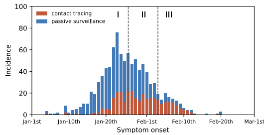
Fig. S3. Incidence of SARS-CoV-2 infections by onset date, for cases captured through contact tracing (red) or passive surveillance (blue). The dashes lines indicate the Phase I, II, and III of epidemic control.
