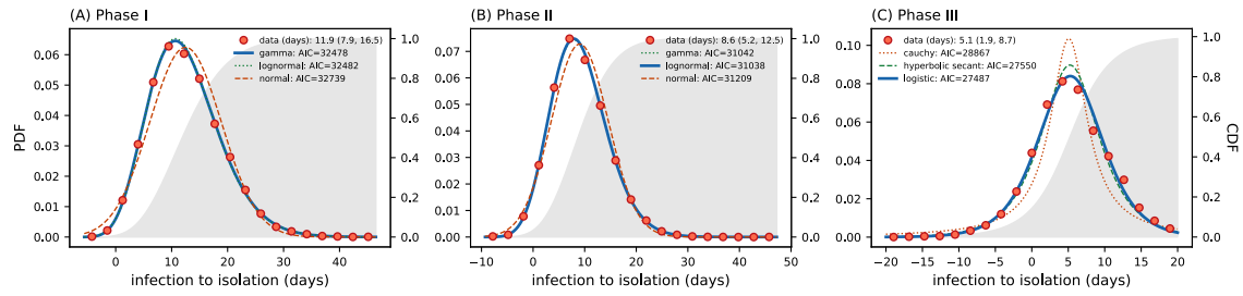
Fig. S5. Same as S3 but focusing on the time from infection to isolation. (A) Phase I of epidemic control (before Jan. 27): time from infection to isolation has a median of 11.9 days with IQR (7.9, 16.5) days (B) Phase II of epidemic control (Jan. 27 – Feb. 4): time from infection to isolation distribution has a median of 8.6 days with IQR (5.2, 12.5) days. (C) Phase III of epidemic control (after Feb. 4): time from infection to isolation distribution has a median of 5.1 days with IQR (1.9, 8.7) days.
