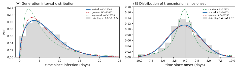
Fig. S6. (A) Distribution of generation interval \tau_{GI}^{adj} adjusted for censoring due to case isolation and quarantine. This represents the distribution that would have been observed in the absence of quarantine and case isolation. The distribution of \tau_{GI}^{adj} has a median of 5.6 days with IQR (3.2, 9.0) days. Grey bars represent data; solid lines represent the Weibull distribution fit to the data (best fit based on AIC score); dashed lines represent gamma and lognormal distributions fitted to the data. (B) Distribution of time from symptom onset to transmission \tau_{OT}^{adj} ; negative values represent pre-symptomatic transmission. Grey bars represent data; solid lines represent the normal distribution fitted to the data (best fit based on AIC score); dashed lines represent Cauchy and gamma distributions fitted to the data.
