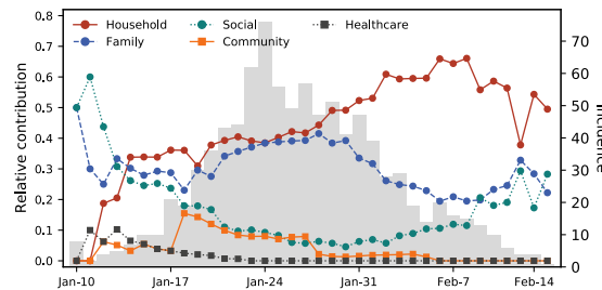
Fig. S7. Trends in the relative contribution of different types of contacts to SARS-CoV-2 transmission. Estimates are averaged over a 10-day moving window. The grey shade in the background indicates the time series of SARS-CoV-2 incidence in Hunan, China.
