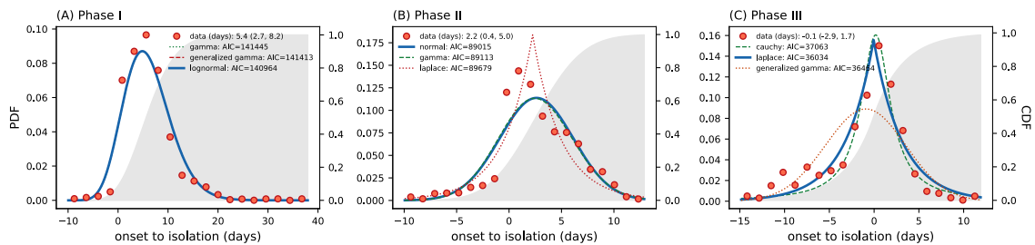
Fig. S4. Distribution of time from symptom onset to isolation in three different phases of epidemic control. Dots are data estimated from the transmission chains, lines are candidate distributions fitted to the data and solid lines distributions fitted best to the data based on Akaike information criterion (A) Phase I of epidemic control (before Jan. 27): time from onset to isolation has a median of 5.4 days with IQR (2.7, 8.2) days. (B) Phase II of epidemic control (Jan. 27 – Feb. 4): time from onset to isolation distribution has a median of 2.2 days with IQR (0.4, 5.0) days. (C)
