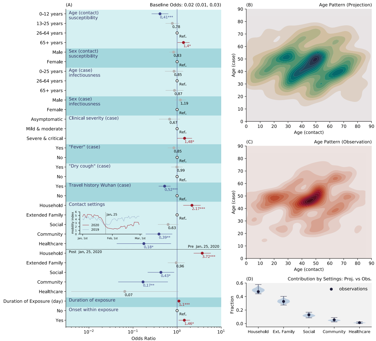
Fig. S1. (A) Individual predictors of transmission risk among close contacts of SARS-CoV-2 infected individuals in Hunan. The predictors of the logistic regression as those indicated on the left (fixed effects) and we also include random effects for individual SARS-CoV-2 infections. Dots and lines indicate point estimates and 95% confidence interval of the odds ratio, numbers below the dots indicate the numerical value of the point estimates; “Ref.” stands for reference category; * indicates p -value <0.05 , ** indicates p -value <0.01 , *** indicates p -value <0.001 . Top inset indicates the within city mobility index in Changsha, Hunan for year 2020 and 2019, provide by Baidu Qianxi (10); dashed line indicates January 25, 2020. (B) Age distribution of projected infector-infectee pairs based on the regression model (average over 100 ensemble projections). (C) Age distribution of observed infector-infectee pairs. (D) The contribution of household, family, social, community, and healthcare contacts to transmission. Dots represent empirical observations and violin plots represents model estimates based on 100 ensemble projections.
