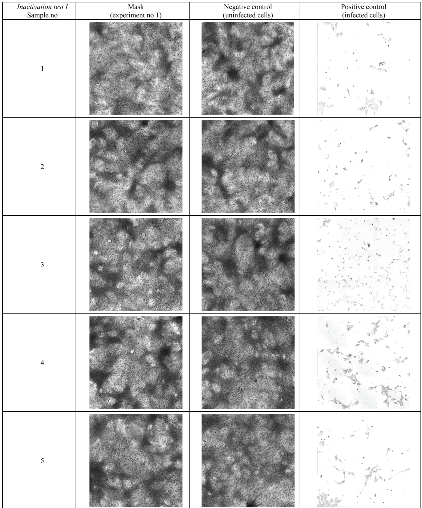
Figure S1. VeroE6 cells at day 6 post infection. VeroE6 cells inoculated with SARS-CoV-2 recovered from paper discs after heat-inactivation (mask #1). VeroE6 growth with complete medium (negative control). VeroE6 cells inoculated with SARS-CoV-2 recovered from paper discs without heat-inactivation (positive control).
