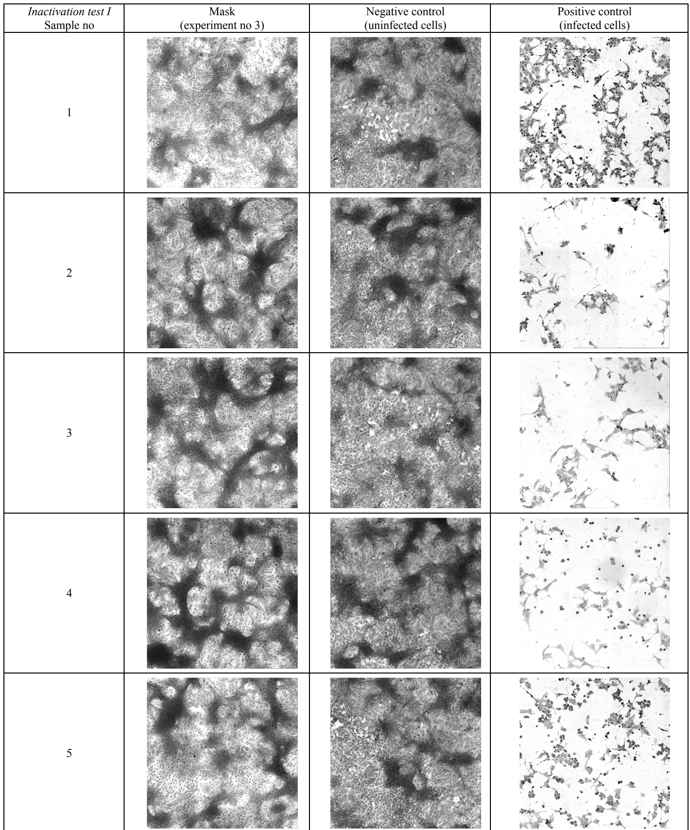
Figure S3. VeroE6 cells at day 6 post infection. VeroE6 cells inoculated with SARS-CoV-2 recovered from paper discs after heat-inactivation (mask #3). VeroE6 growth with complete medium (negative control). VeroE6 cells inoculated with SARS-CoV-2 recovered from paper discs without heat-inactivation (positive control).
