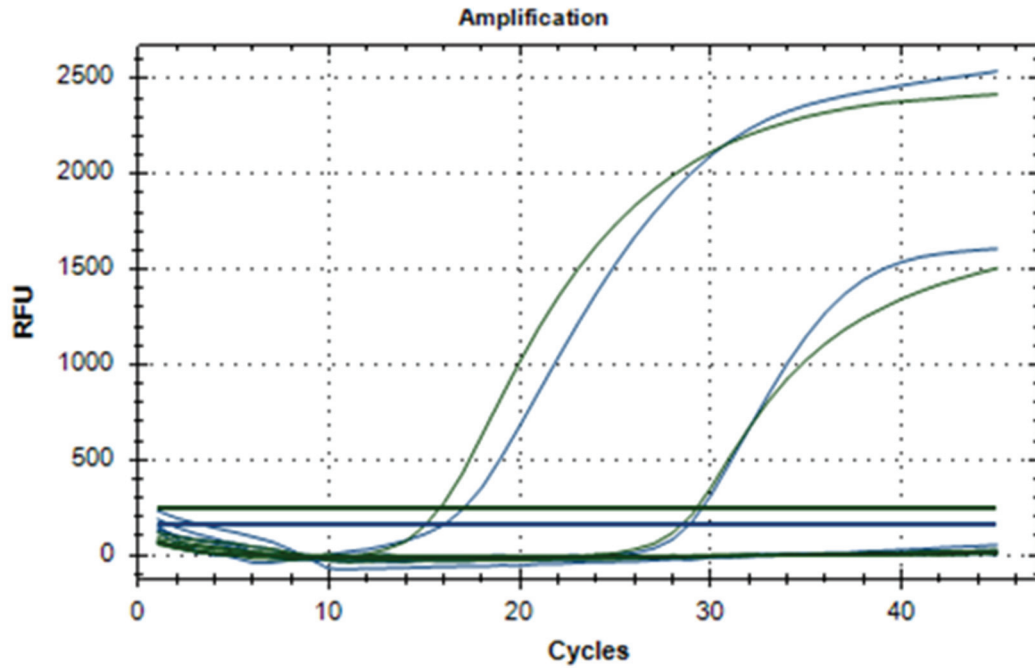
Figure S5 qRT-PCR amplification of viral RNA Methods from the experiment shown in Fig. S4. After centrifugation, 200 \mu l of supernatant were extracted using the « High Pure Viral Nucleic Acid » kit from Roche following the supplier's recommendations. qRT-PCR was performed following indications of the supplier (SARS-CoV-2 RT-qPCR Perkin Elmer). Briefly, 6 \mu l of reactional mix were mixed with 14 \mu l of a 1/10 dilution of each sample. Amplification of positive and negative controls supplied in the kit were also performed. Two viral genes, ORF1ab-gene and N-gene, were targeted. According to the supplier, Ct \leq 32 for ORF1ab or \leq 35 for N-gene are considered as positive. Ct \geq 40 or undetermined are negative. Figure S5 presents a representative experiment of qRT-PCR. Supernatant of cells infected with positive control (untreated virus) were positive with Ct of 15.80 and 16.10 for ORF1ab-gene and N-gene respectively. All other samples, uninfected cells, cells infected with heat treated samples, negative control of the kit, were undetected. Positive controls of the kit is detected with Ct \leq 32 as expected : 29.25 for of ORF1ab and 28.92 for N-gene.
