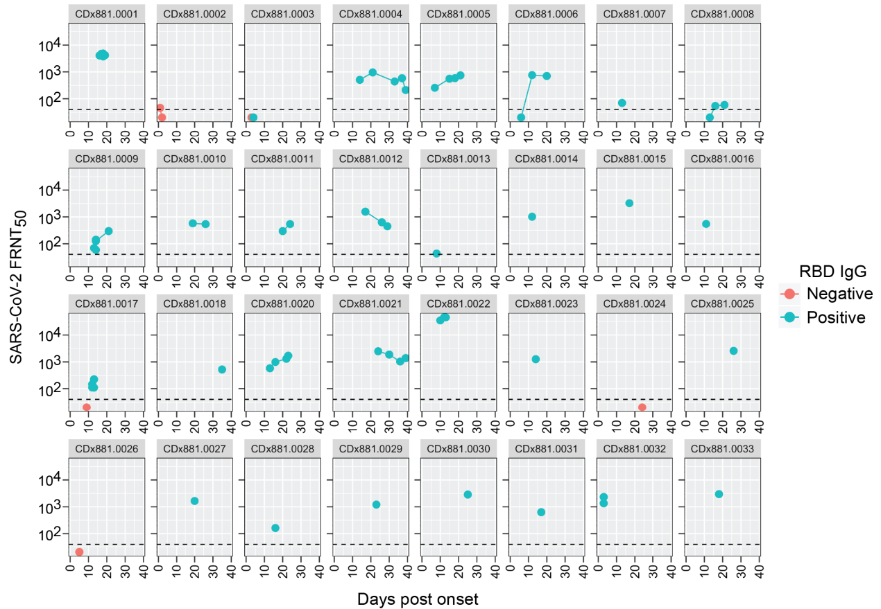
11 12 Figure S3 | SARS-CoV-2 neutralization in COVID-19 patients. Focus reduction (by 50%) 13 neutralization titers (FRNT 50 ) was determined by serial dilution of serum samples from COVID- 14 19 patients taken at different times post onset of symptoms. RBD-IgG reactivity is indicated for 15 each sample. FRNT 50 cutoff is indicated by dotted line and was set at 1:50 which was the 16 lowest dilution tested. FRNT 50 -negative samples were assigned a titer of 1:20.
