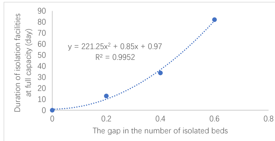
Supplementary Figure 1. Curves of the duration of isolation facilities at full capacity under different gaps in the number of isolated beds.
