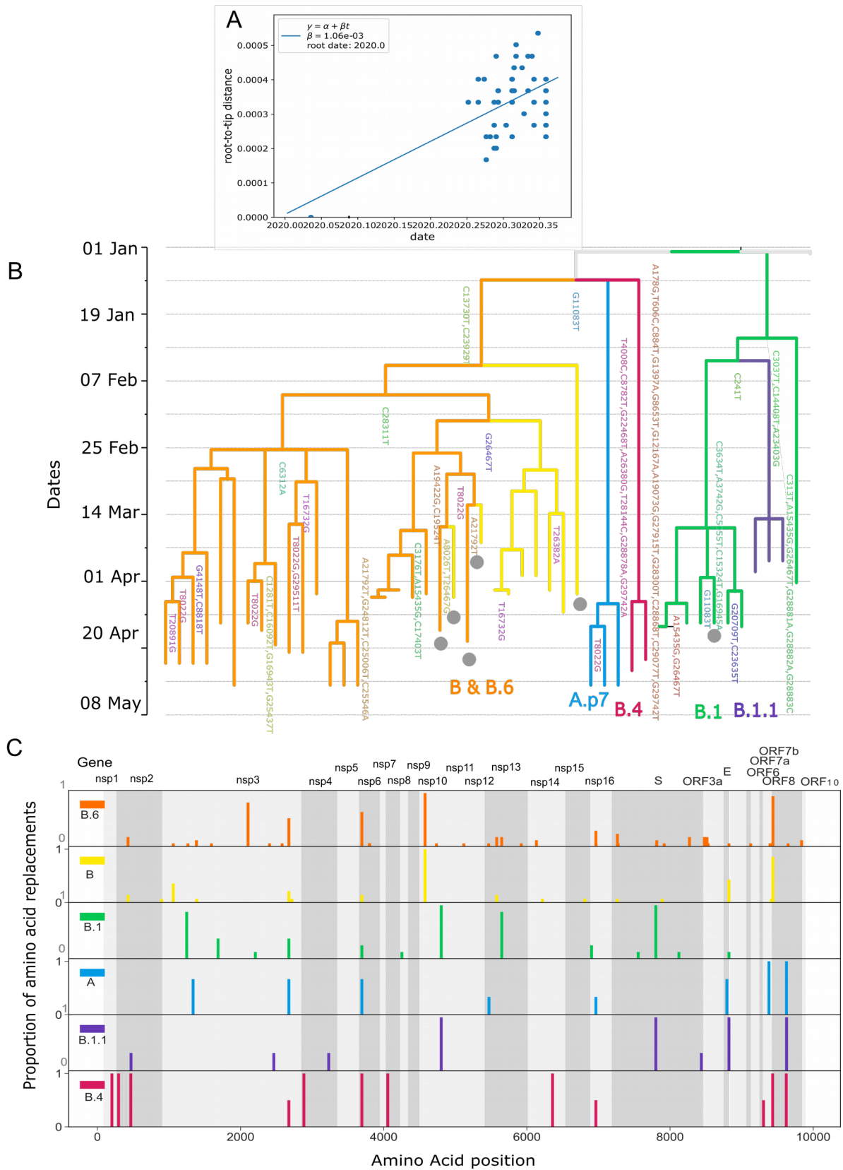
Supplementary Figure 2- A . Root to tip regression analysis of sequences used in this study. Mutation rate is estimated at 1.062e-03 mutations/site/year with r^2 = 0.28 . Note: While the temporal signal in this data is weak, analysis of larger datasets by others is suggestive of a molecular clock. B . Time scaled maximum likelihood tree of genomes from this study. Coloured circles represent sequences from symptomatic individuals. Mutations/SNPs at each node are labelled in the tree. All changes are with respect to the reference genome. C . Frequency of amino acid replacements in different lineages. Details are provided in Supplementary Table 3
