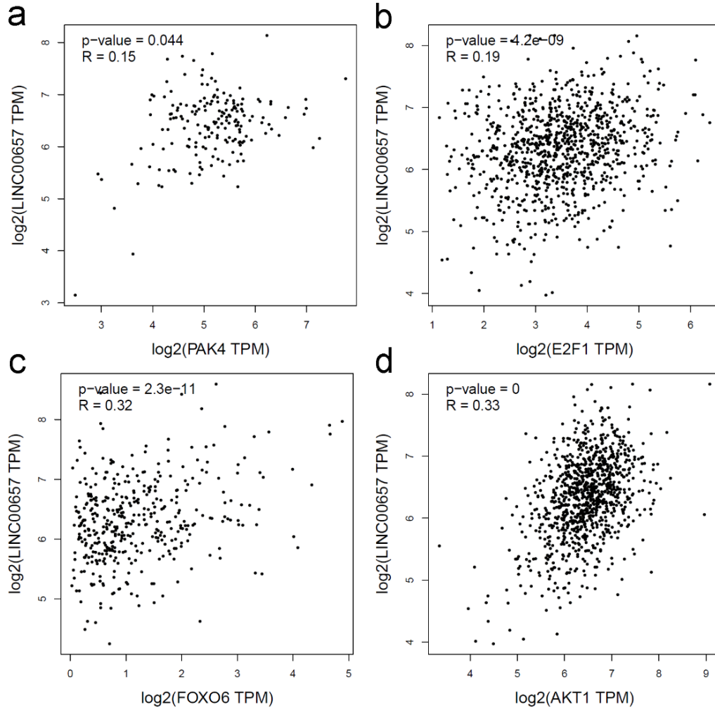
Supplementary Figure S4. Correlation analysis between gene expression levels. (a) Correlation between NORAD and PAK4 expression; (b) Correlation between NORAD and E2F1 expression; (c) Correlation between NORAD and FOXO6 expression; (d) Correlation between NORAD and AKT1 expression.
