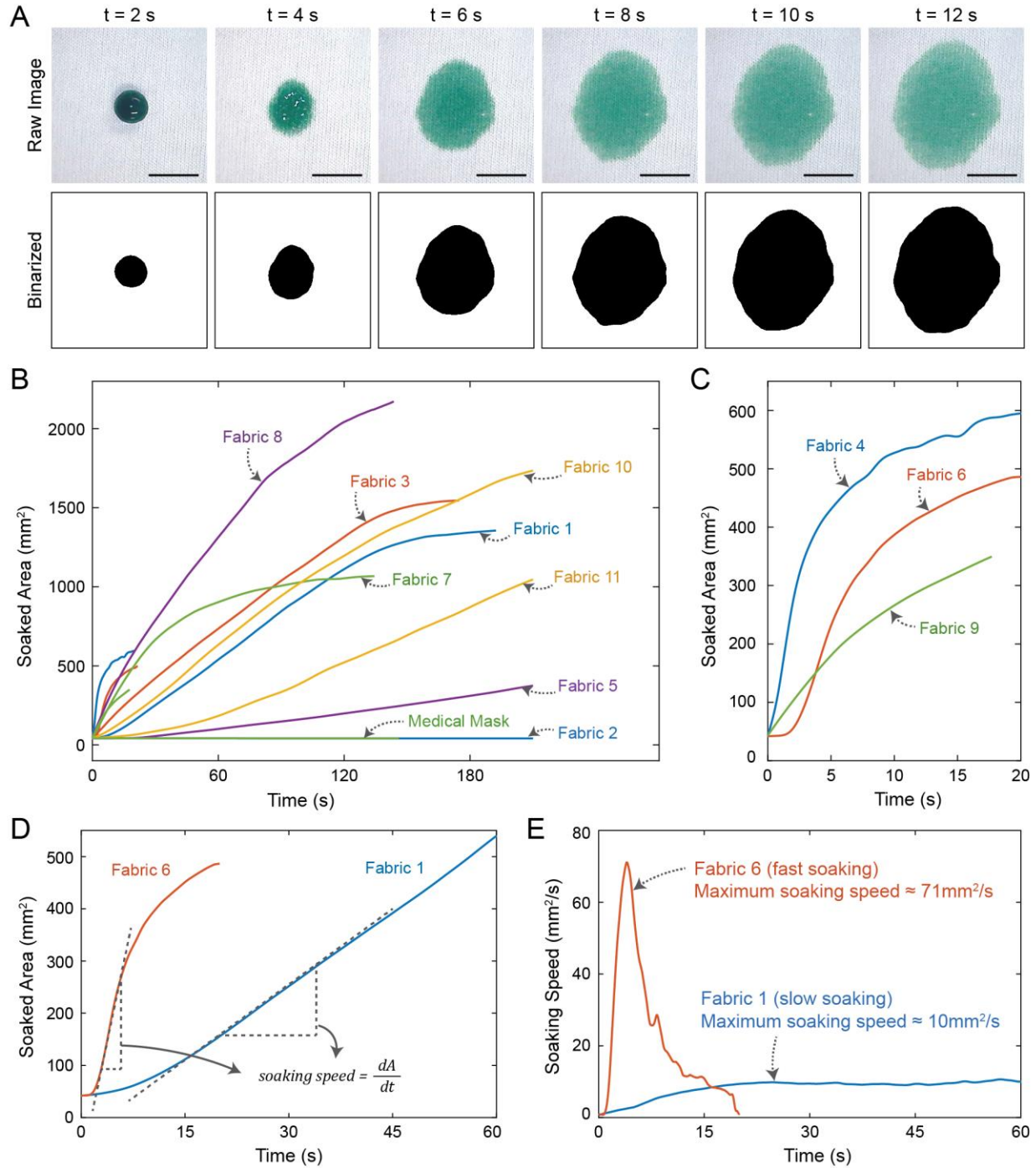
Figure S4. Measurement of water soaking speed. (A) Top row: Snapshots from water soaking test on T-shirt fabric (fabric 6) with green food coloring added for contrast. Scale bars: 10 mm. Bottom row: Corresponding binary images which were used to quantify soaked area. (B, C) Soaked area plotted against time for all fabrics tested. (D) Soaking speed is calculated as the time derivative of soaked area. Area vs. time plots for a fast soaking sample (fabric 6) and relatively slow soaking sample (fabric 1) are shown as examples. (E) Soaking speed vs. time plotted for fabrics 6 and 1.
