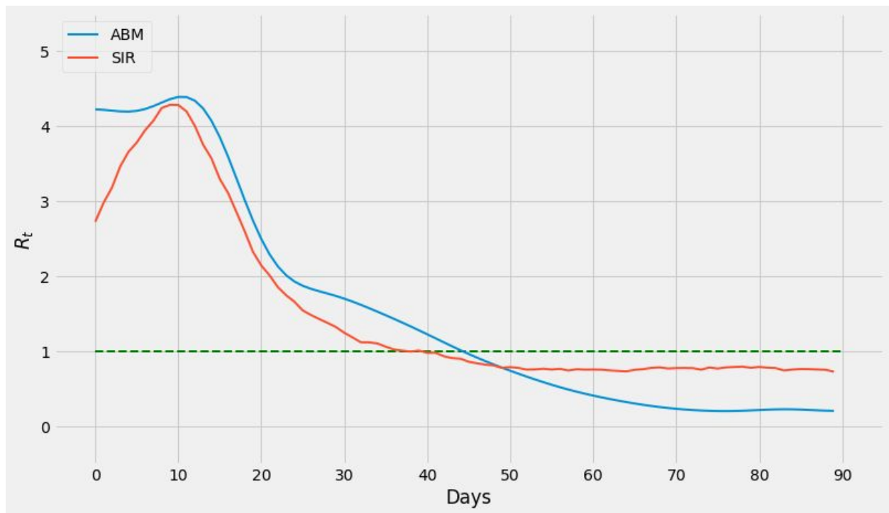
Figure 1: R_t curves by ABM model with scaled down population (blue) and SIR model with full population (red) of NYC. The blue curve appears to be similar to the red curve with an RMSE value of 0.4626, although converging to zero sooner than the red curve because of the smaller size of population.
