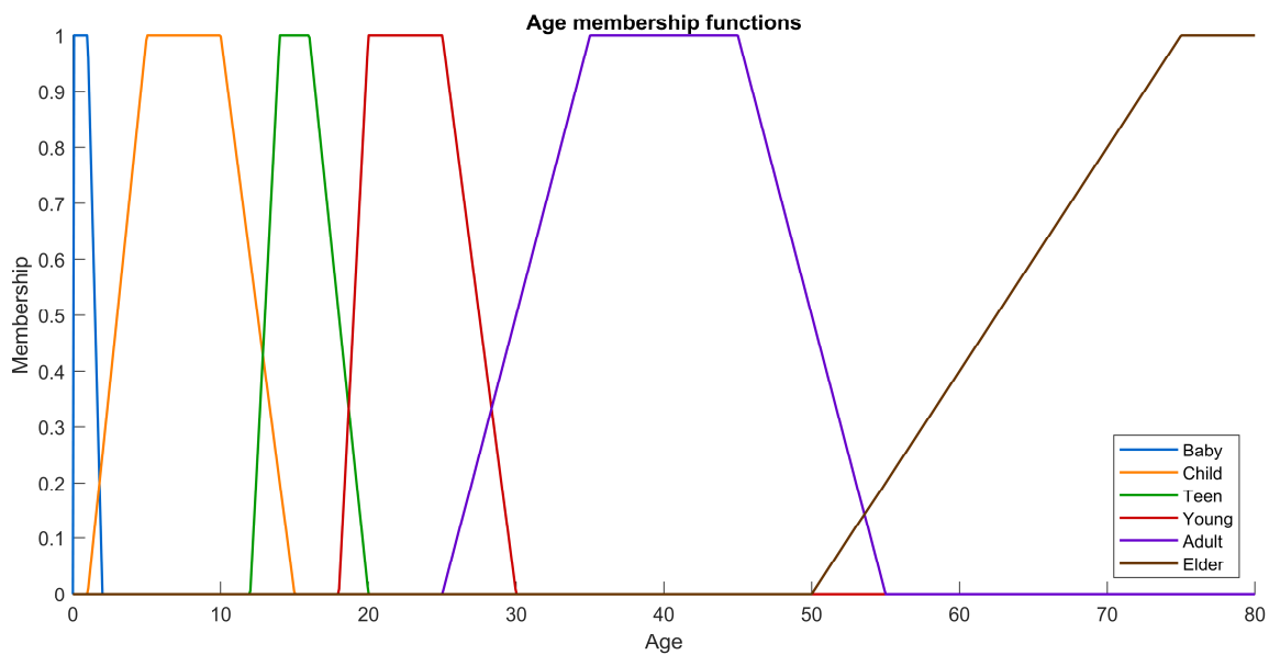
Figure 1. Piecewise linear functions representing age group membership.
