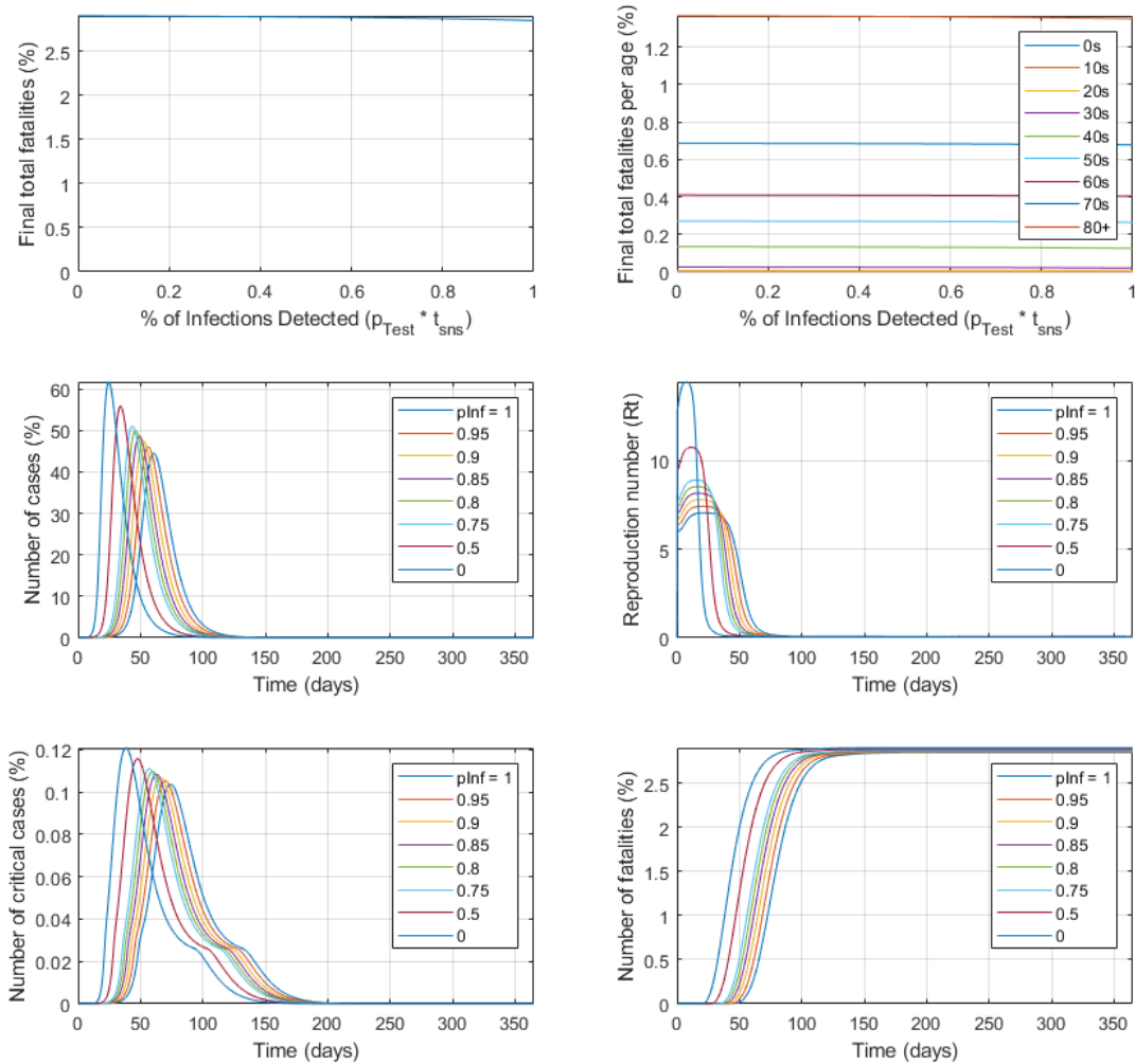
Figure S8b. Impact of extensive testing of the infected pre-symptomatic individuals only that leads to modified isolation factor respect to their default r_{\text{fi}} values (Table S3), on the final total number of fatalities (top left); the final total number of fatalities per age group (top right) as well as for the different time course profiles of the total active cases (middle left); reproduction number ( R_t ) (middle right); the number of critical cases (bottom left) and the number of fatalities (bottom right). Numbers are in percentage of the total population of all ages.
