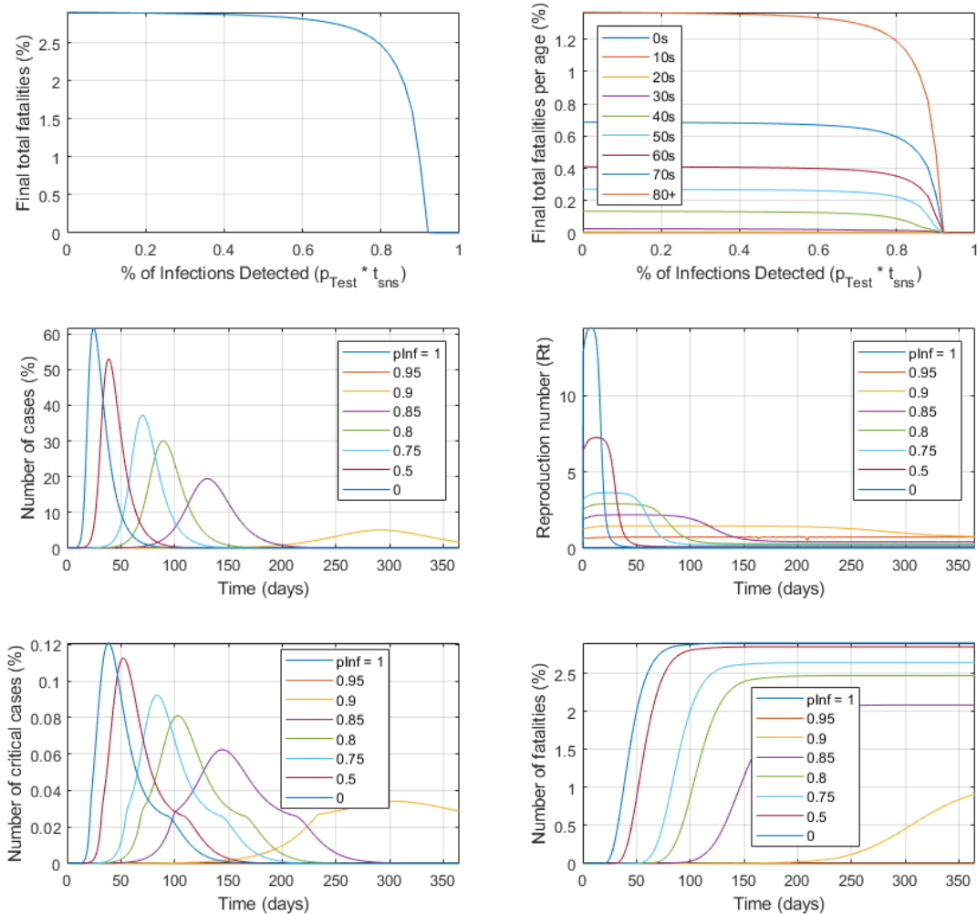
Figure S8c. Impact of extensive testing of both infected symptomatic and pre-symptomatic individuals that leads to modified isolation factor respect to their default rfi values (Table S3), on the final total number of fatalities (top left); the final total number of fatalities per age group (top right) as well as for the different time course profiles of the total active cases (middle left); reproduction number ( R_t ) (middle right); the number of critical cases (bottom left) and the number of fatalities (bottom right). Numbers are in percentage of the total population of all ages.
