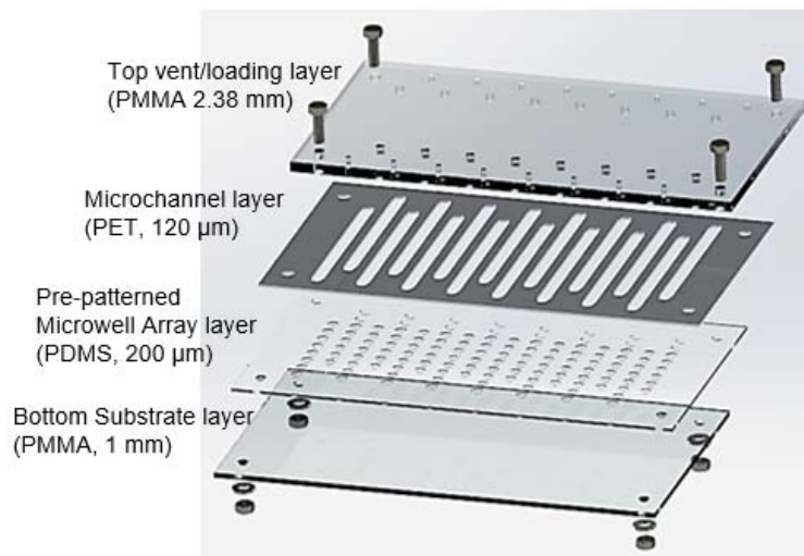
Figure S1. Fabrication of disposable PED-ELISA microfluidic cartridge. The chip contains two polymethyl methacrylate (PMMA) layers (top venting and bottom substrate layers), a thin polydimethylsiloxane (PDMS) layer (200 \mu\text{m} ), which contains fL-sized microwell arrays for digital assay, and a polyethylene terephthalate (PET) thin film (120 \mu\text{m} ) with microfluidic channels fabricated by laser cutting.
