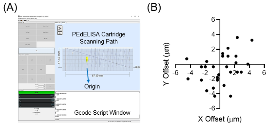
Figure S3. (A) User-interface of the Universal Gcode Sender for automated PEdELISA assay image scanning (B) Characterization of bi-directional motion control accuracy by repeatedly scanning and imaging the designated microarray on the chip. Bi-directional repeatability with a positional error of less than 5 \mu\text{m} was achieved.
