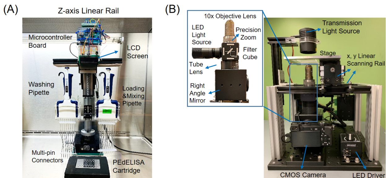
Figure S2. PEdELISA assay platform comprising two modules: (A) programmed fluidic handling module with Arduino controlled linear rail and multi-channel pipettes. (B) customized low-cost 2-axis fluorescence scanning module with a consumer-grade CMOS camera.
