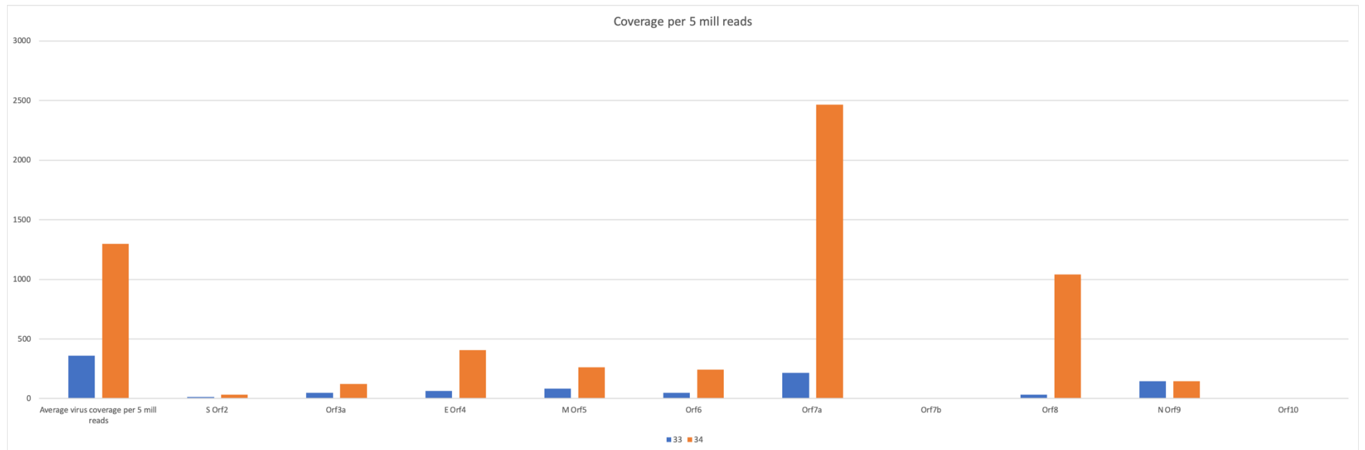
Supplementary Figure S1: Average coverage per 5 million reads for samples 33 and 34.
