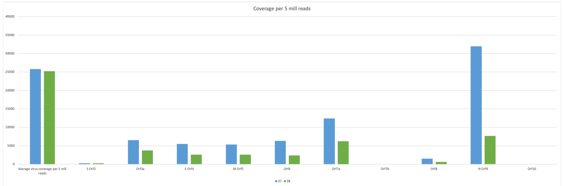
Supplementary Figure S2: Average coverage per 5 million reads for samples 37 and 38.
