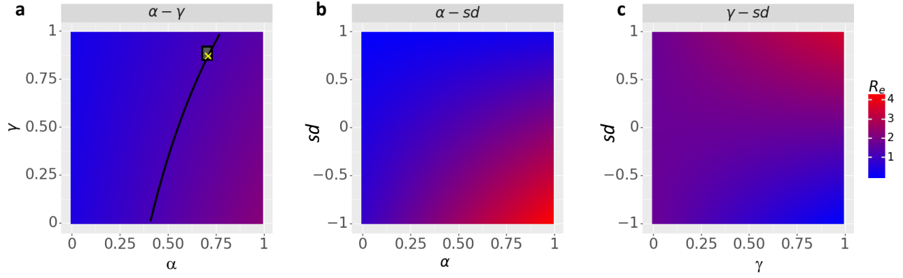
Figure S13. The dependency of R_e on model parameters \alpha and \gamma and social mobility sd . All other variables are held constant with values represented in Table S1 for state BW. \alpha - \gamma : The impact of \alpha and \gamma on R_e . The value of sd is set to sd = 0.35 . Black curve represents the constant R_e = 1.21 . The box represents the interval of inferred parameters that have the maximum likelihood and the yellow 'X' mark shows the parameter combination used for estimation ( \alpha = 0.71 , \gamma = 0.89 ). \alpha - sd : The impact of \alpha and social mobility sd on R_e . Note that sd is not a model parameter. \gamma - sd : The impact of \gamma and social mobility sd on R_e .
