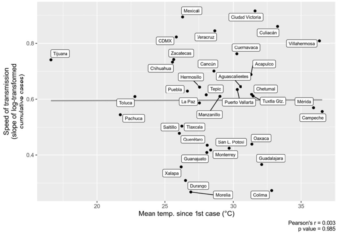
SM Figure 1: Relation of rate of transmission of COVID-10 to temperature
