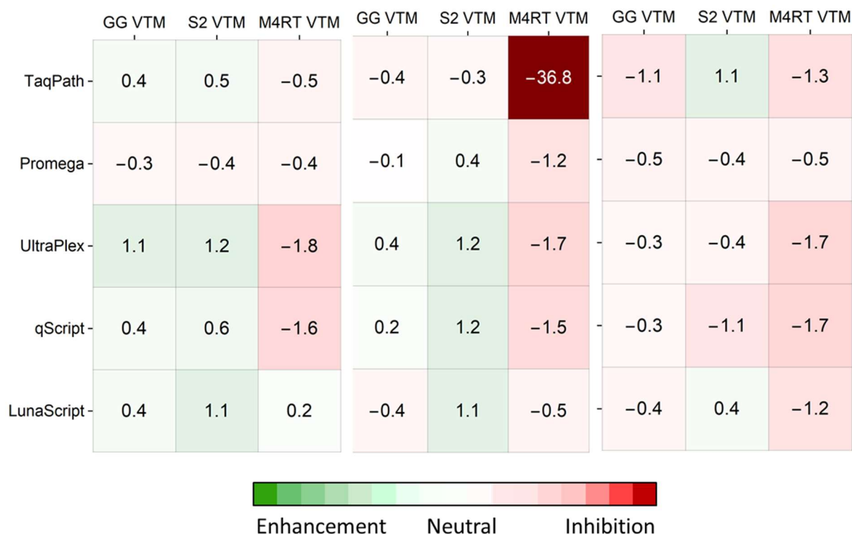
Figure S2. Impact of VTM on the CDC singleplex test. The TaqPath MM was the least inhibitor tolerant while both the UltraPlex and qScript MMs were the most tolerant and even showed some amplification enhancement. The amplification enhancement and inhibition are reduced or entirely removed when diluted VTM is tested. The data presented are fold-change in Ct values between RNA spiked in VTM and control reactions of RNA spiked in 10 mM Tris buffer, pH 8. If a condition did not have a Ct value it was set to 45 to generate a difference in Ct measure. Conditions marked with a “✦” indicate at least one of the replicates did not have a Ct value after 45 cycles indicating complete amplification inhibition. All reported values are averages of N=3 per condition. The M4RT VTM resulted in the most inhibition across all dilutions and master mixes tested. A. Impact of 1:10 VTM dilution in 10 mM Tris, pH8, B. 1:100, and C. 1:1000.
