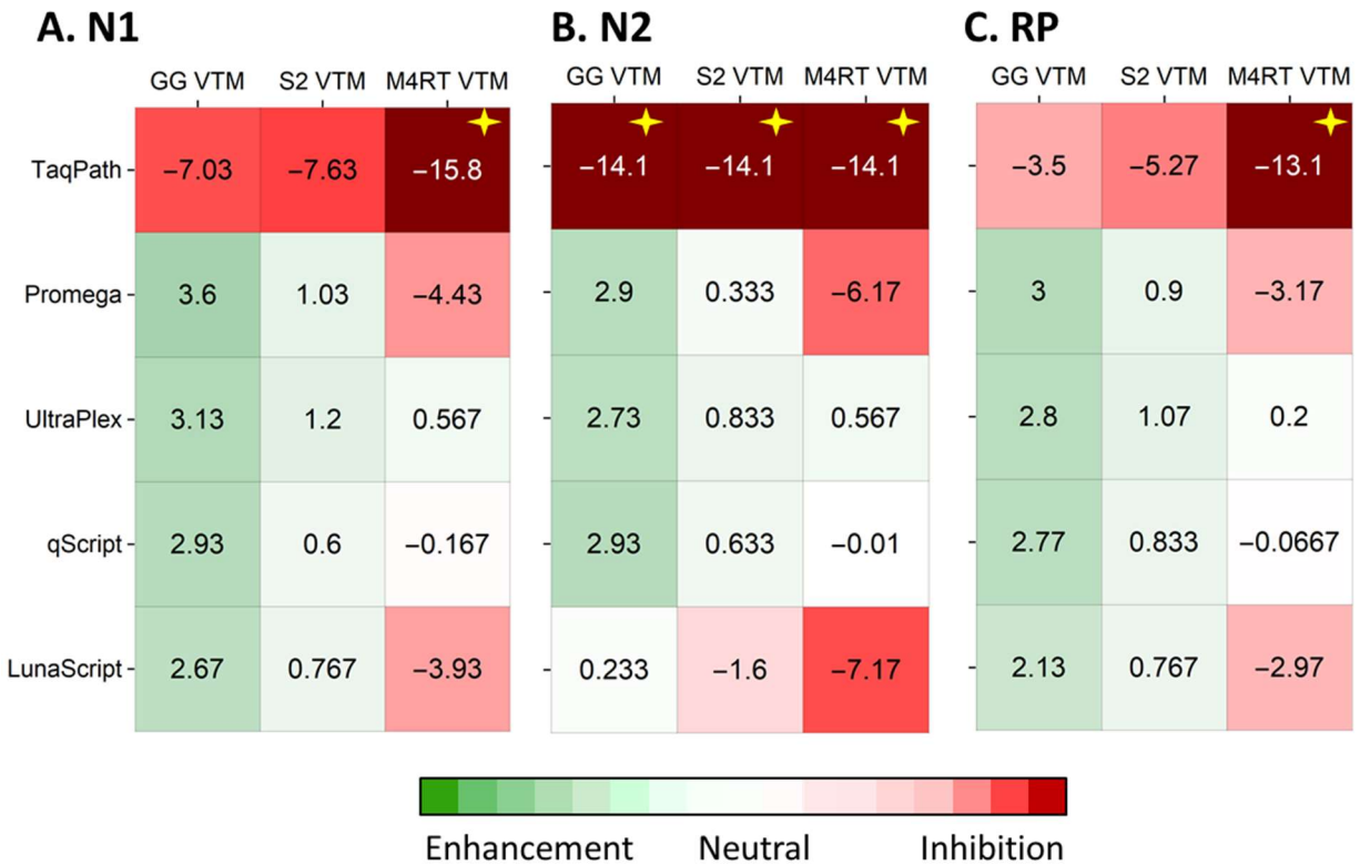
Figure S1. The \Delta C_t values used to determine the fold-change for the studies exploring the impact of VTM on the CDC singleplex test. These data correspond to the fold-change data presented in Figure 2 in the main manuscript. If a condition did not have a C_t value it was set to 45 to generate a difference in C_t measure. Conditions marked with a “✦” indicate at least one of the replicates did not have a C_t value after 45 cycles resulting in complete amplification inhibition. All reported values are averages of N=3 per condition. The SARS-CoV-2 and human RNA were kept constant at 820\text{ c}/\mu\text{L} and 2000\text{ c}/\mu\text{L} , respectively. A. Impact on SARS-CoV-2 N1 target, B. N2 target, and C. the human RP target.
