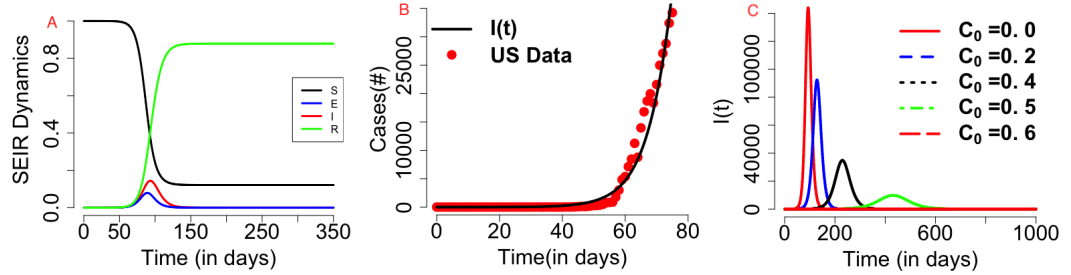
Figure 1: Epidemiological dynamics in the absence of control measures (a), fit of the model to United States data (b), and effects of social distancing measures in flattening the epidemic curve (c). Time series for susceptible (S), latent (E), infected (I) and recovered (R) individuals from the model is shown on the left. Time window on the right runs from 21-01-2020 to 05-04-2020 and compares case prevalence in model to corresponding US data. All parameters are at baseline parameter values (Table 1) and initial conditions S(0) = 1000000 and I(0) = 1 , except for control parameters in (a) that are set to zero in the absence of control.
