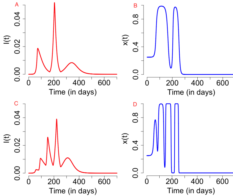
Figure 4: Time series plot of infection, I(t) and social, x(t) dynamics, (upper) for \kappa = 10 and (bottom) for \kappa = 80 .
