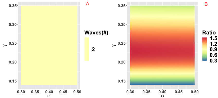
Figure 2: Parameter plane showing model dynamics as they vary with changes in the rate \gamma at which the infectious period ends and the rate \sigma at which the latent period ends, for the number of COVID-19 waves (a) and the ratio of peak height of the second wave to the first wave peak (b). Other parameters are at baseline values (Table 1).
