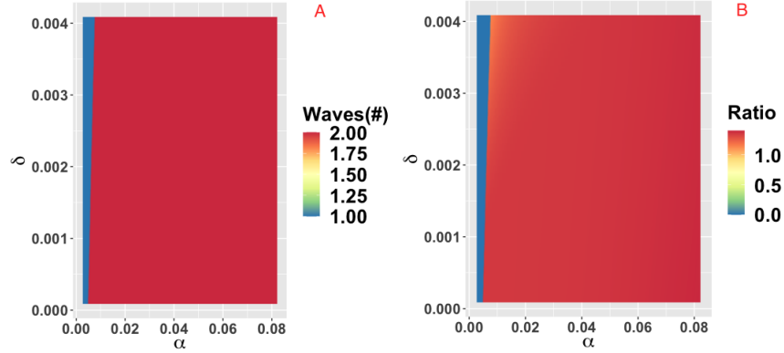
Figure 3: Parameter plane showing model dynamics as they vary with changes in the rate \alpha at which socio-economic losses accrue and the rate \delta at which socio-economic losses are discounted, for the number of COVID-19 waves (a) and the ratio of peak height of the second wave to the first wave peak. Other parameters are at baseline values (Table 1).
