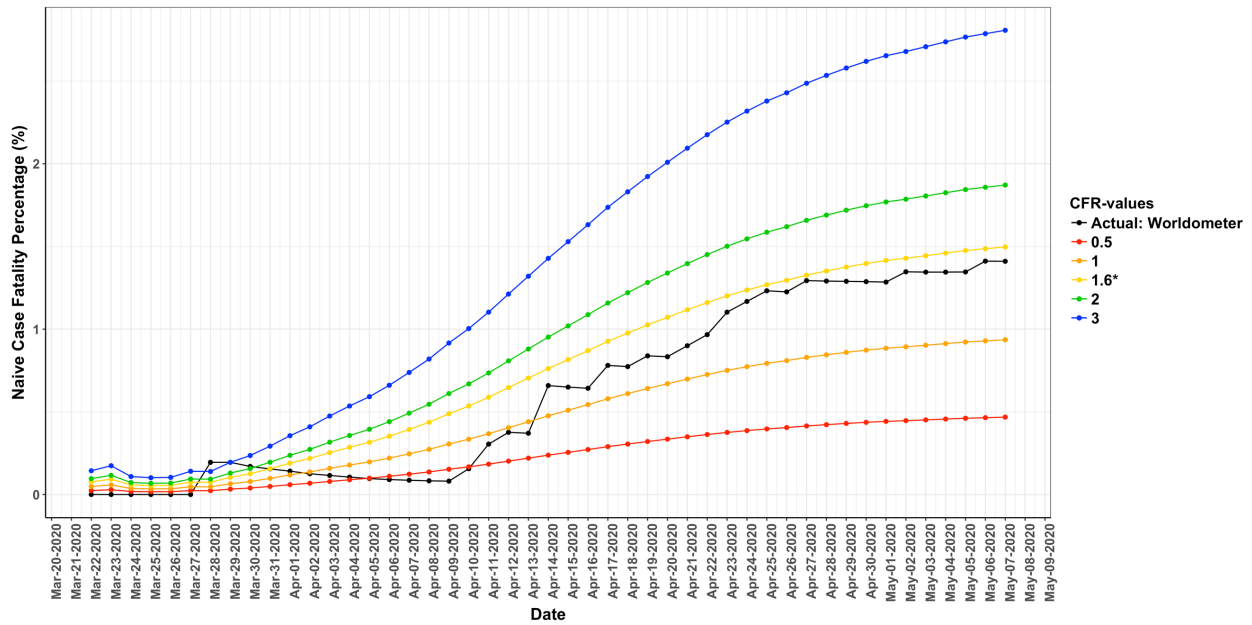
Figure 5. Simulated nCFR(t) and N_D(t) curves for New Zealand. The simulated curves shown were calculated using a corrected CFR of 0.50, 1.0, 1.6 (the closed case nCFR ), 2.0, and 3.0. The reported data is shown in black.
