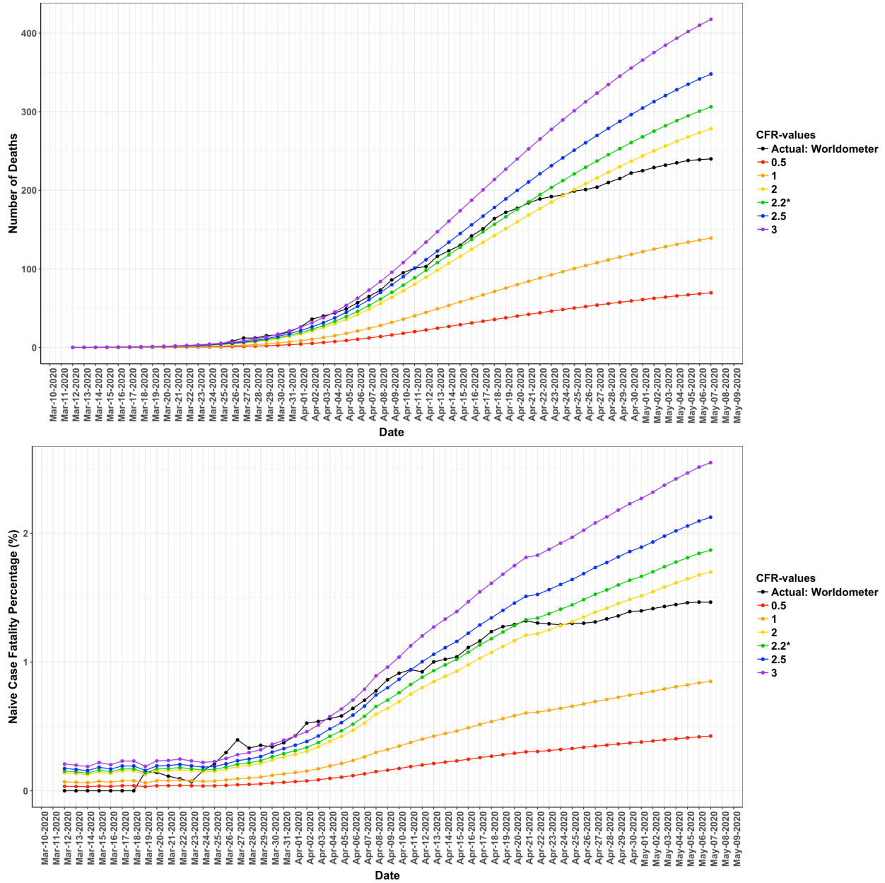
Figure 4. Simulated nCFR(t) and N_D(t) curves for Israel. The simulated curves shown were calculated using a corrected CFR of 0.50, 1.0, 2.0, 2.2 (the closed case nCFR ), 2.5, and 3.0. The reported data is shown in black.
