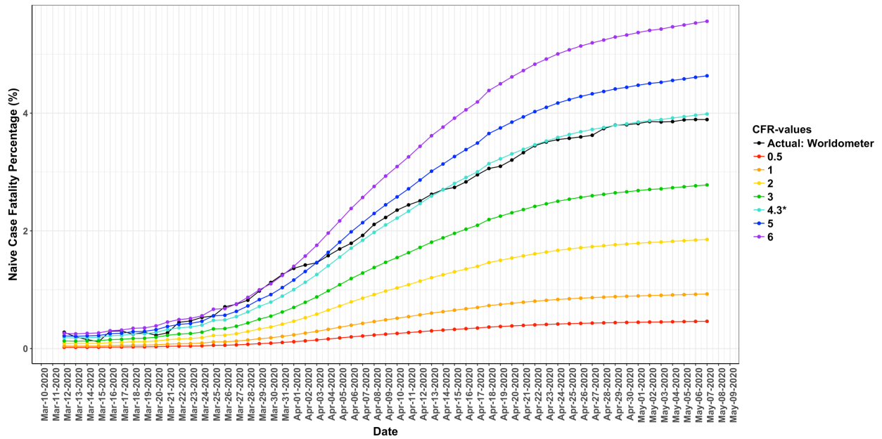
Figure 2. Simulated nCFR(t) and N_D(t) curves for Austria. The simulated curves shown were calculated using a corrected CFR of 0.50, 1.0, 2.0, 3.0, 4.3 (the closed case nCFR ), 5.0, and 6.0. The reported data is shown in black.
