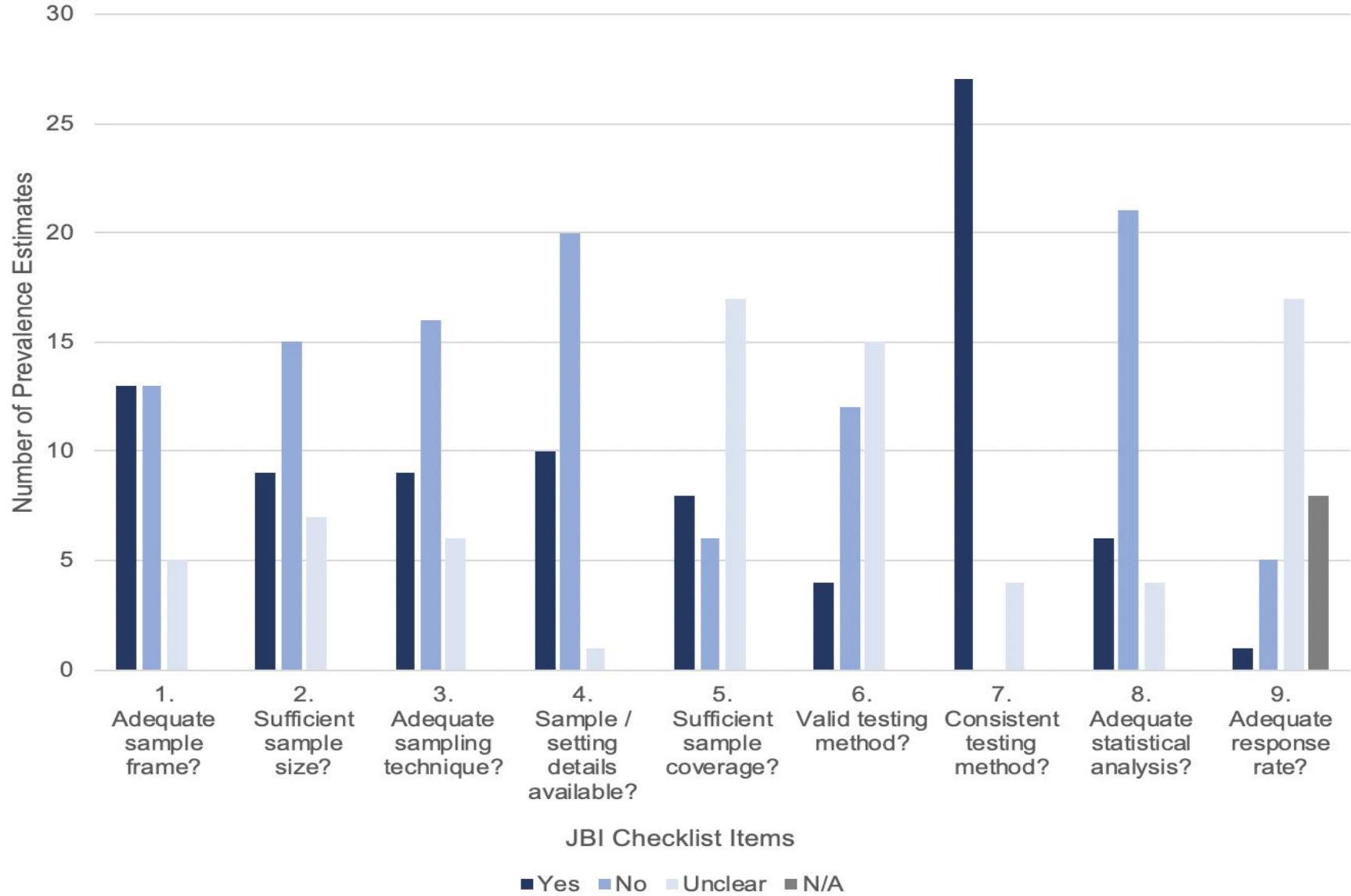
Supplemental Figure 3 Summary of critical appraisal items for prevalence estimates.
