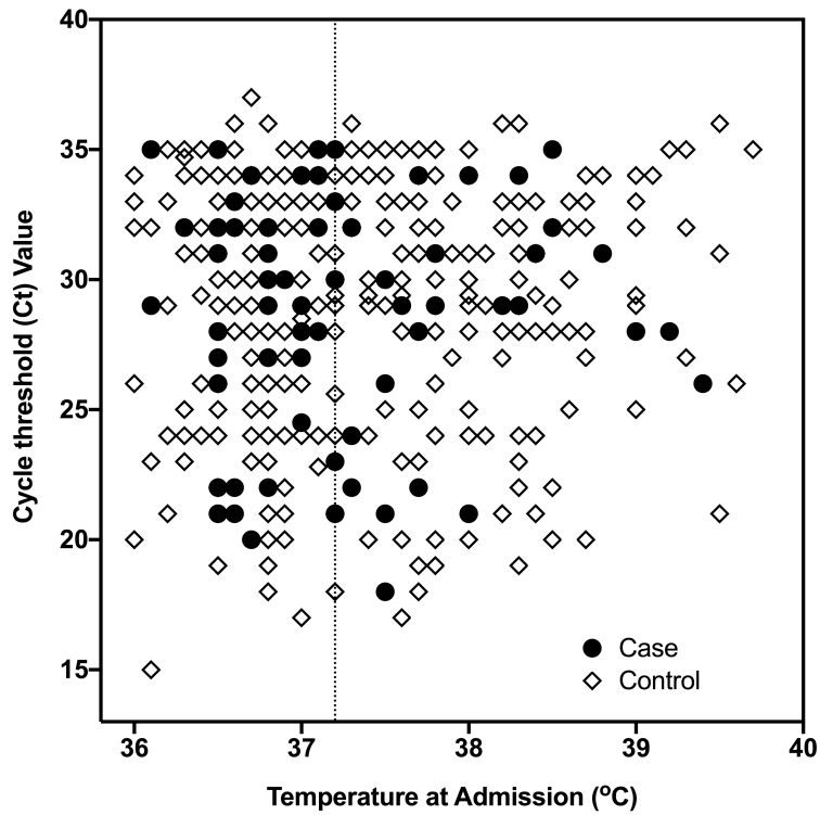
Supplementary Figure 7. This scatterplot demonstrates the relationship between SARS-CoV-2 RNA cycle threshold (Ct) value and body temperature at admission for patients with (i.e. the case group defined by nasopharyngeal swab PCR positivity; solid circles) and without (i.e. the control group; open diamonds) recurrence of PCR positivity. The vertical dotted line represents the threshold of high body temperature ( > 37.2\text{ }^{\circ}\text{C} ).
