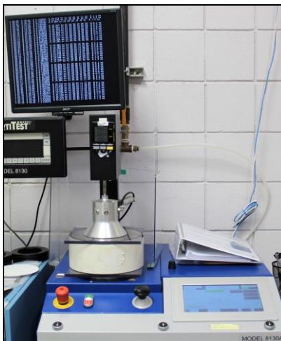
Figure 5. Typical setup for mask under test
