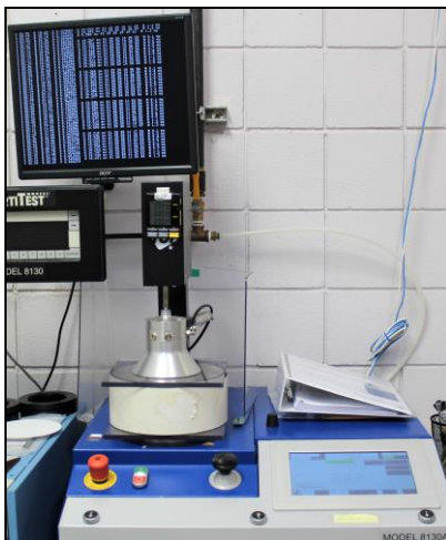
Figure 3. Typical setup for mask under test
