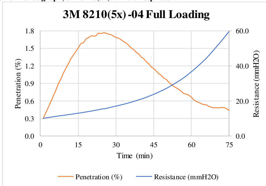
Filter performance graph, 3M 8210(5x)-04 N95 respirator.
