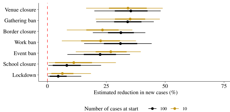
Fig. 6 Estimated reduction (posterior mean as dots with 80% and 95% credible interval as thick and thin lines, respectively) in the number of new cases (in %) for each non-pharmaceutical intervention (NPI) by varying the number of cases at start. Compared are 100 (main analysis) and 10 cases at the start of the analysis.
