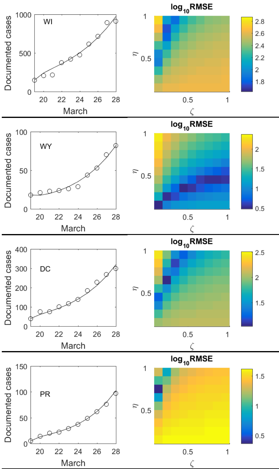
Figure S2. Daily observation of documented active COVID-19 cases (circle) is compared with the best-fit model (line). The color maps show the corresponding combination of \zeta and \eta that gives rise to the minimum RMSE
