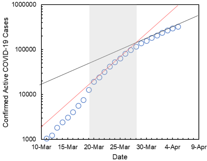
Figure S1. Daily confirmed active COVID-19 cases in the United States between March 10 and April 7.
