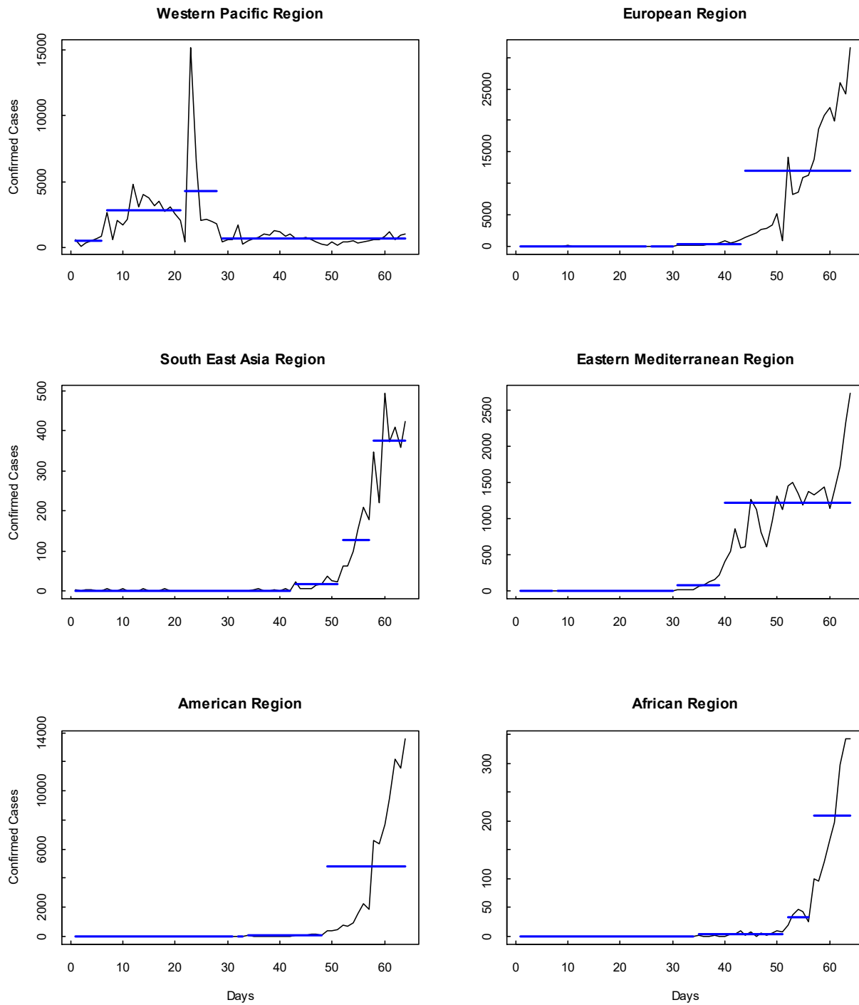
Extended Fig. 5: Same as Extended Fig. 4 except for CPD based on mean and variance
