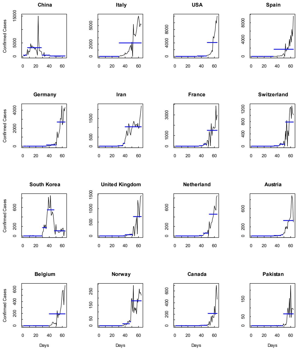
Extended Fig. 7: Same as Extended Fig. 6 except for CPD based on mean and variance
