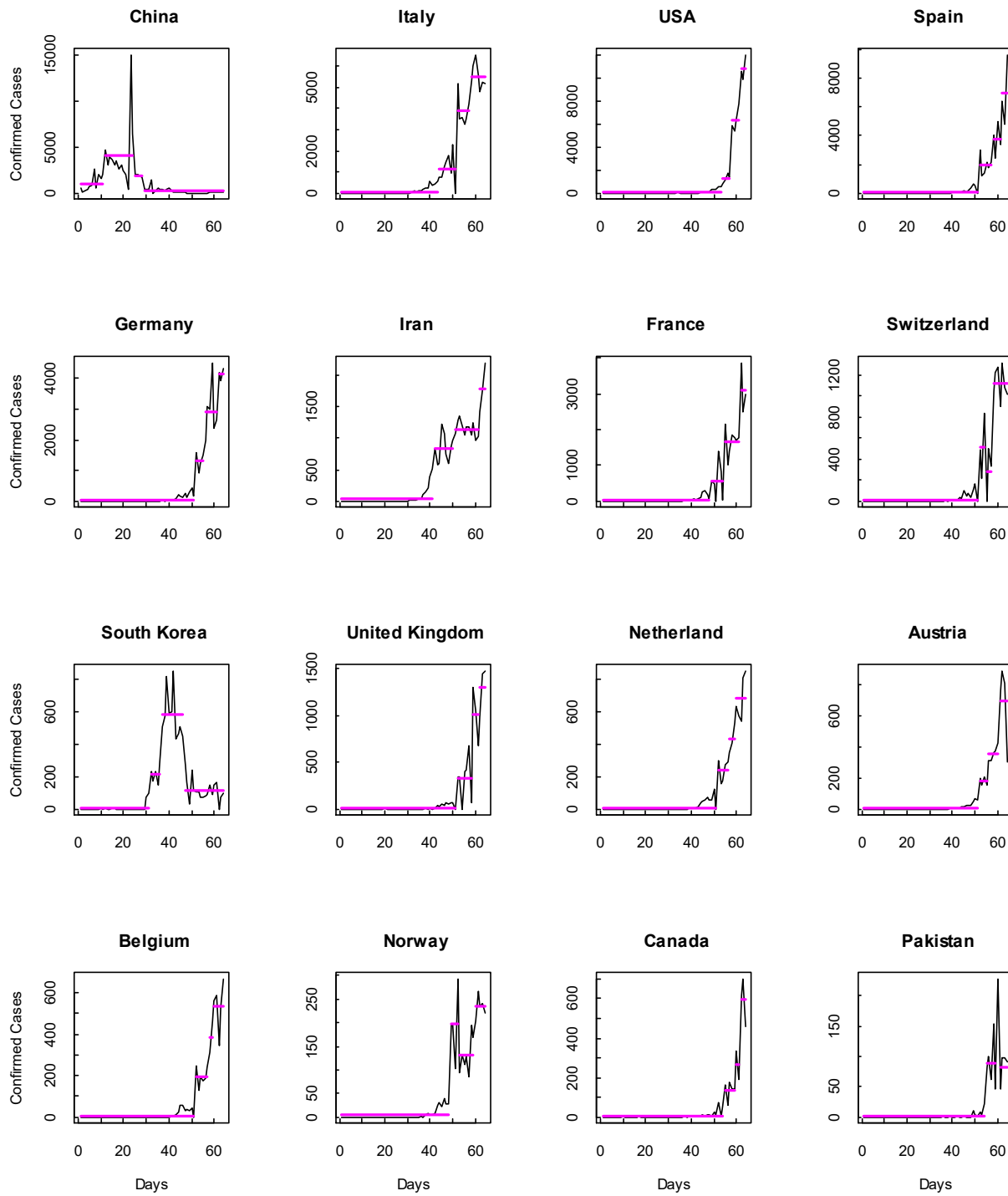
Extended Fig. 6: Multiple CPD based on mean at country scale
