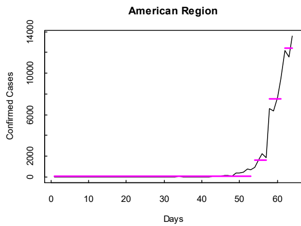
Extended Fig. 4: Multiple CPD based on mean at regional scale
