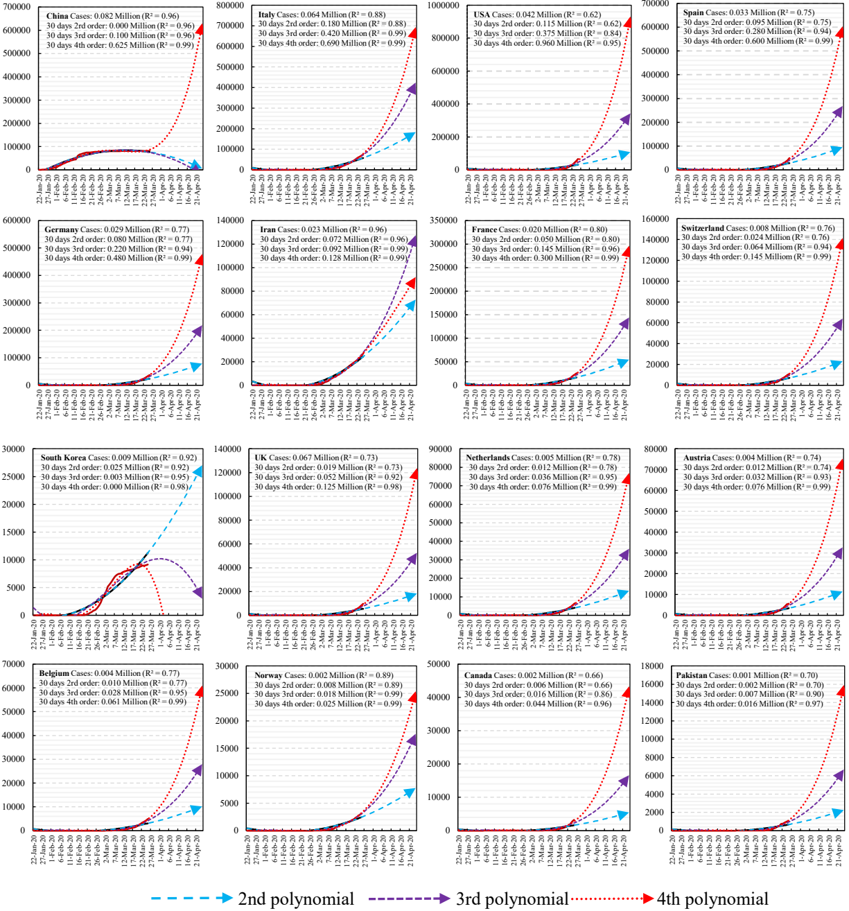
Extended Fig. 10: Selected countries projected infected population based on 2nd, 3rd and 4th order polynomial curve fitting.
