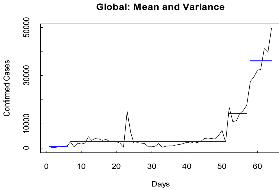
Extended Fig. 8: Global scale multiple CPD.
