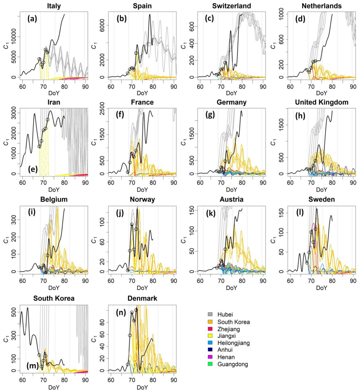
Fig. S5. Empirical scenarios simulations (variable C_1 )
