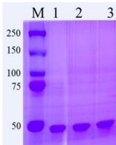
Supplementary figure S1. SDS-PAGE of the purified recombinant nucleocapsid antigen, M band indicates the marker, 1-3 band are the purified recombinant nucleocapsid protein.
