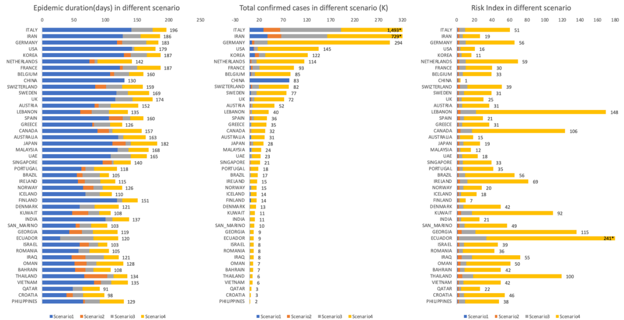
Fig. S2 Forecasted duration, cumulative cases of outbreak end and risk of top 44 outbreak countries in the world.
