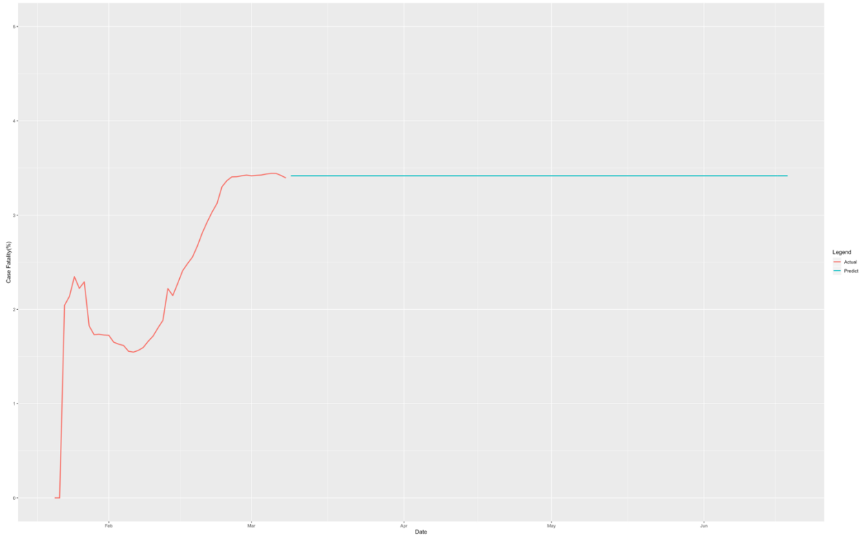
Fig. S4 Case-fatality curve for the world.
