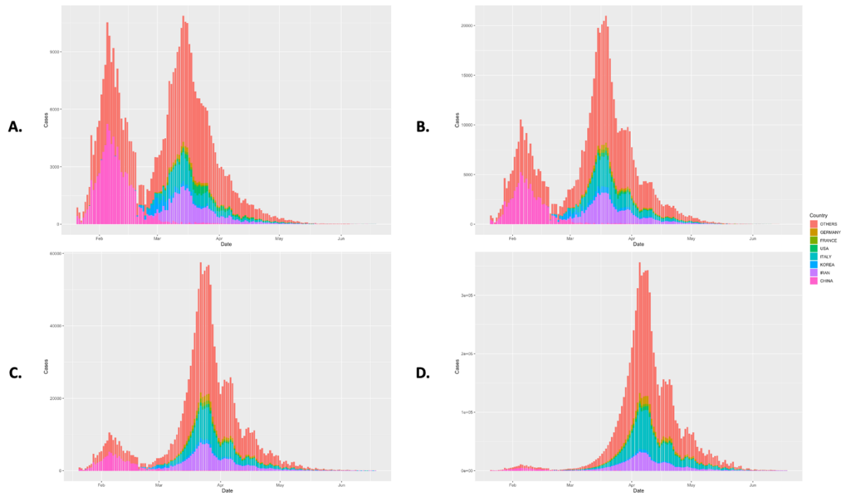
Fig. S3 Time-case plot of the top seven infected countries: China, Iran, Italy, Germany, South Korea, USA, France and all other countries. (A) Time-case plot under intervention scenario 1; (B) Time-case plot under intervention scenario 2; (C) Time-case plot under intervention scenario 3 and (D) Time-case plot under intervention scenario 4.
