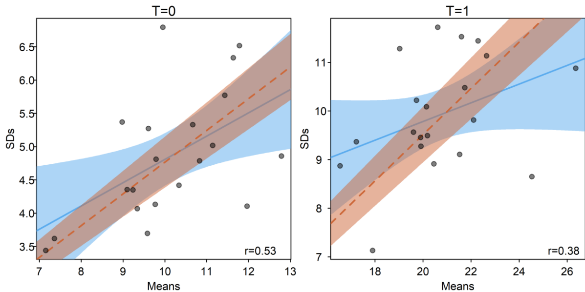
Figure A 1: Plot of mean outcome vs SD for scenario 1. The correlation coefficient is given as r , in the bottom right of each plot. Blue solid line: the unadjusted regression line and 95% confidence intervals. Orange dashed line: the unadjusted regression line, forced through the origin, with 95% confidence intervals.
