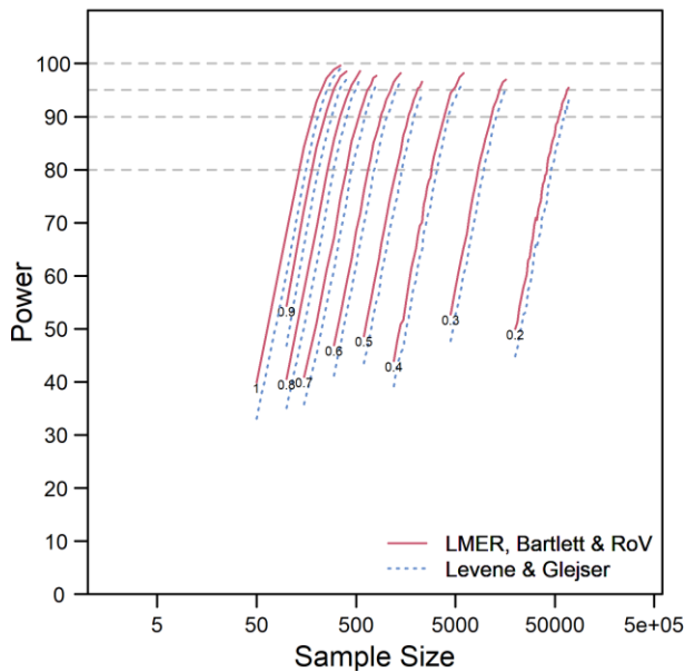
Figure A 5: Plot of sample size ( N ) vs the power to detect difference in variances between the two arms for scenarios with different standard deviations in the two arms (varying \sigma_1 : see methods). The numbers on the lines indicate the value of \sigma_1 . Grey dashed horizontal lines indicate power = 0.8, 0.9, 0.95 and 1.0. 10,000 simulations were performed for each N . (Figure A 6 shows individual panels for each \sigma_1 , without a logged x-axis.)
