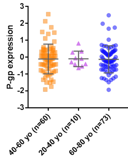
P-gp expression by age at diagnosis
