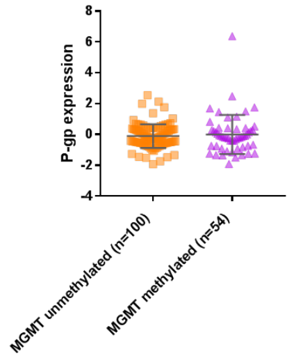
P-gp expression by MGMT status
