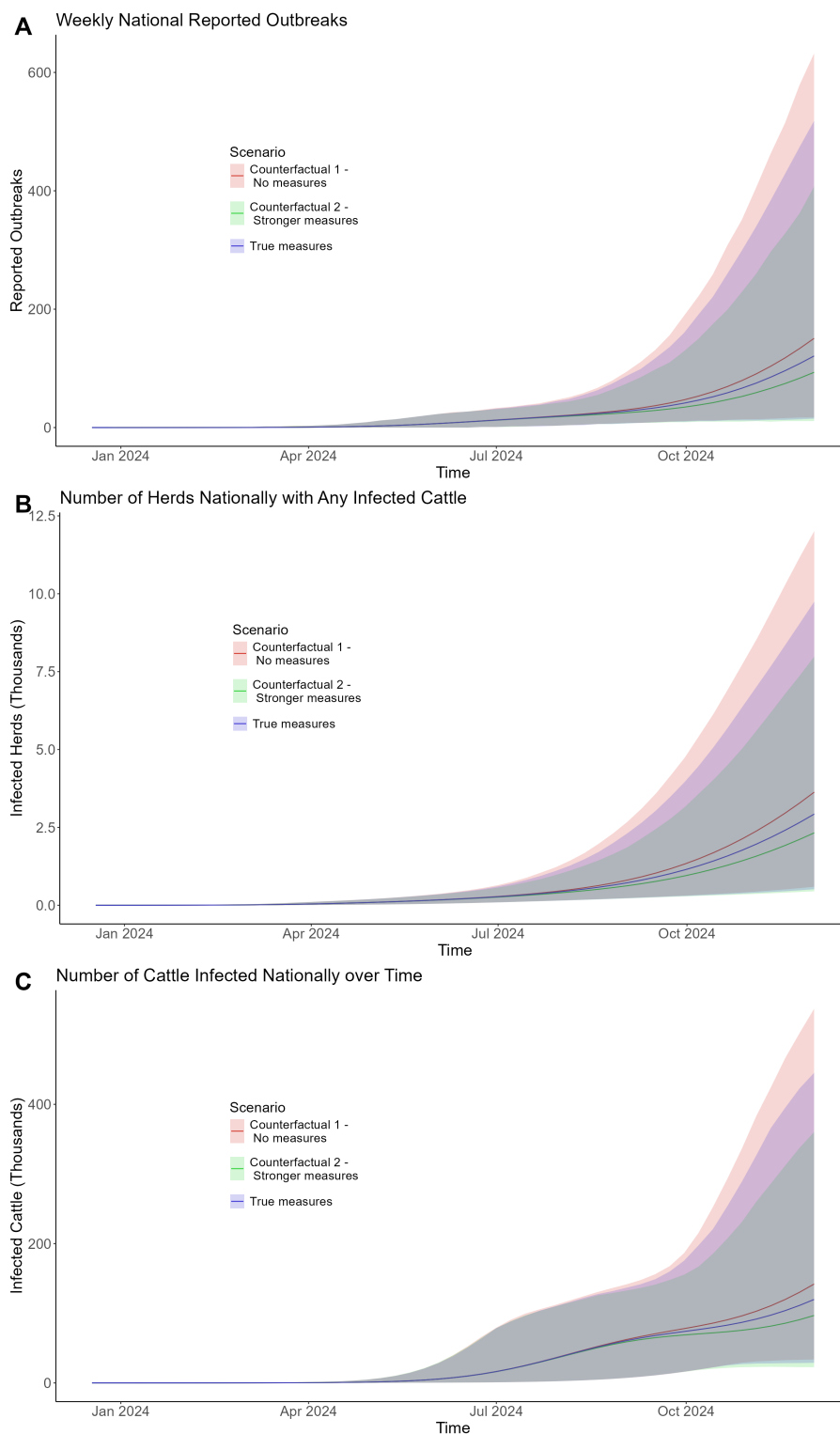
Figure 5: Testing intervention counterfactuals. (A) The number of new reported outbreaks weekly. (B) The number of herds nationally with any infected cattle. (C) The total number of infected cows nationally over time. Solid lines show simulation mean. Shaded regions show 95% CrI. Blue depicts baseline model assumptions. Red depicts the scenario with no border testing. Green depicts border testing of up to 100 cows, implemented 28 days earlier, on April 1st 2024.
