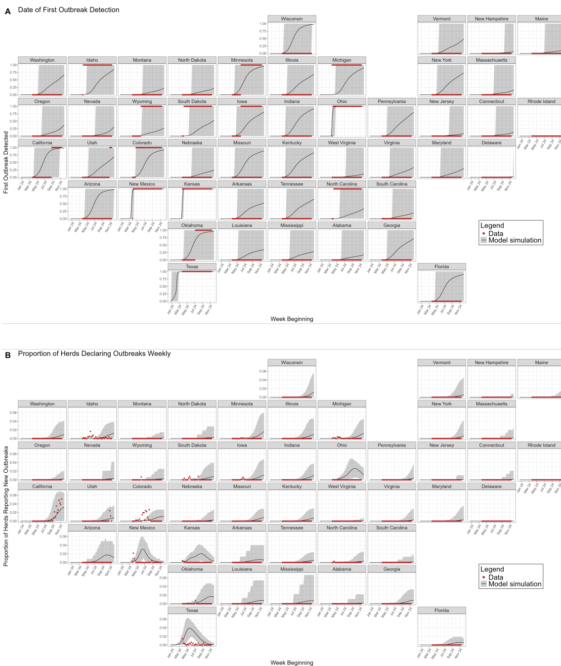
Figure 2: Model simulations. (A) shows the date at which the first outbreak is detected in a state. (B) shows the proportion of herds in each state which report new outbreaks per state each week, accounting for under-reporting. Red points depict data. The black line depicts the model mean, the shaded grey region depicts the 95% credible interval (95% CrI).
