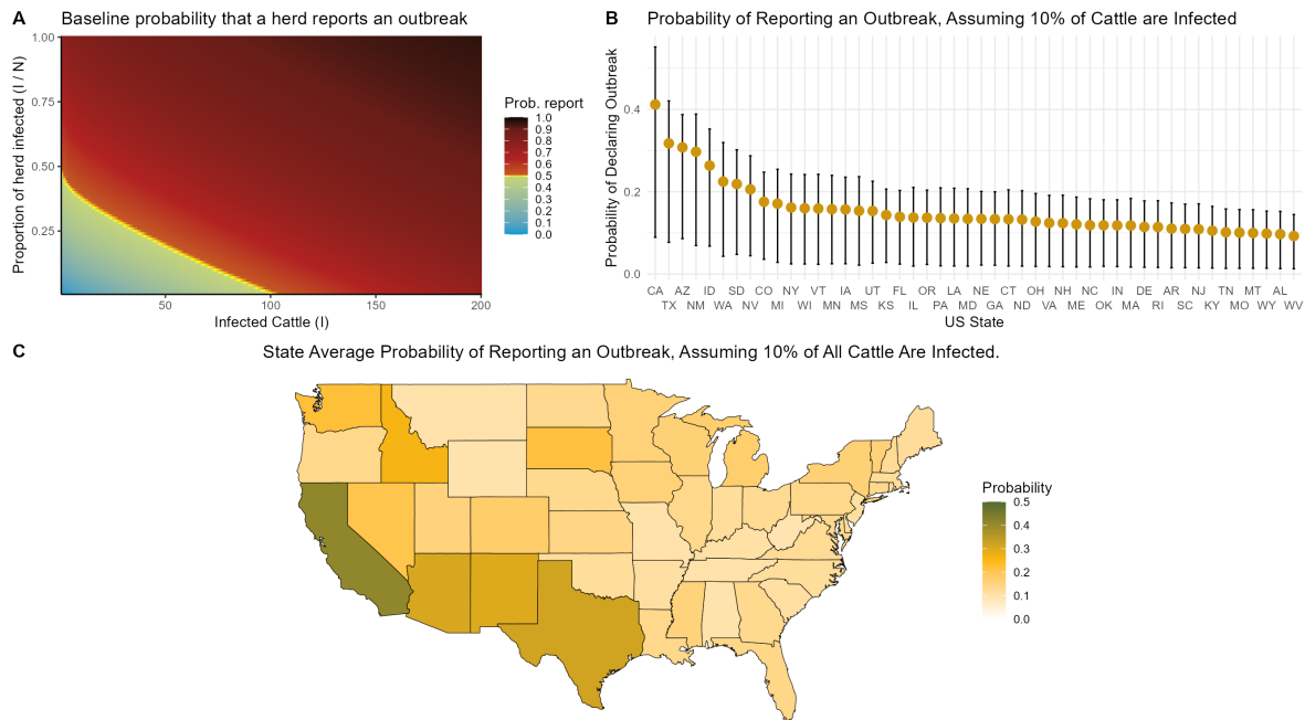
Figure 3: Ascertainment rate assumptions. (A) shows how the modeled baseline probability of reporting an outbreak depends on the number and proportion of infected cattle in a herd. Our model assumes that the probability that an infected herd reports an outbreak depends on the size of the holding, and the number of infected cattle on that date. Panel (B) shows the mean and 95% CrI per-herd probability a herd reports an outbreak by US state, assuming every herd has 10% of its cattle infected. The credible interval captures the variation in herd sizes and the posterior distribution of the ascertainment rate parameter. Panel (C) maps the mean values shown in (B).
