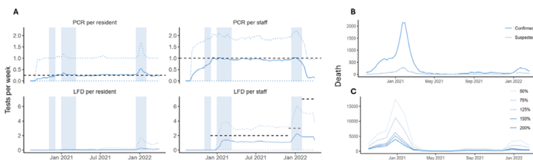
Fig. 2 (A) Average reported numbers of tests per person per week in England for adult social care staff and residents. Blue vertical bars show periods when care homes were closed to visitors (with the exception of visiting for palliative care/end-of-life and named essential caregiver visits) due to government closure policies and community-wide lockdowns. (B) Confirmed and suspected COVID-19-related deaths of residents in 14,805 English care homes studied. (C) The model-projected total COVID-19-related deaths under hypothetical testing levels relative to historical levels. Each line corresponds to a different counterfactual scenario when the numbers of tests were at the levels shown on the right-hand side of the panel relative to the historical levels, e.g. 50% means that the number of tests was decreased by 50% from its factual level.
