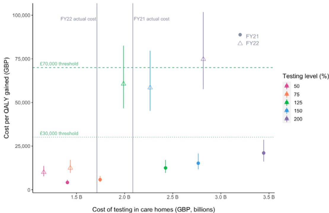
Fig. 3. Cost effectiveness of actual testing levels in adult social care homes in England compared with various hypothetical levels of testing. The whiskers represent the cost-effectiveness ranges using a minimum QALY of 4.98 per death averted and a maximum of 8.8 per death averted. The points falling below the GBP 70,000 willingness to pay threshold are considered to be cost effective. The points to the right of the vertical lines indicate testing volumes that would be more expensive than the actual strategy was (125%, 150%, and 200% of the actual testing volume).
