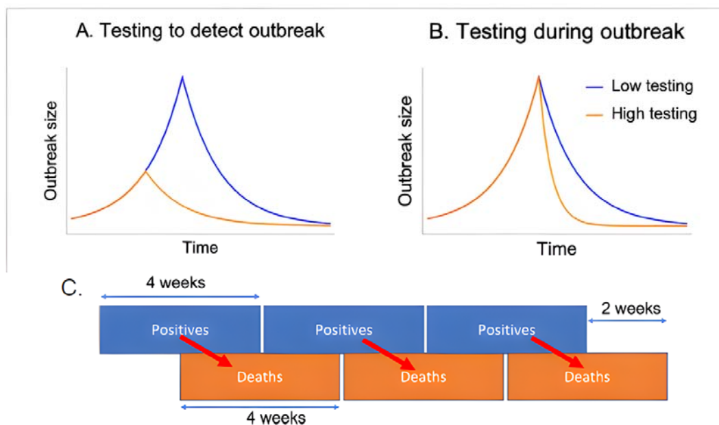
Fig. 1 Characterising the two pathways through which our models assume testing influences outbreak dynamics (A and B) and design of positives-to-deaths regression (C). Panel (A) shows that higher levels of testing are associated with outbreaks being detected earlier, when they are smaller in size (leading to more rapid outbreak control). Panel (B) shows that higher levels of testing during outbreaks are associated with more rapid control of outbreaks. Panel (C) shows the link between our dependent variable (COVID-19-related deaths) and testing variables, one of our independent variables, in our regressions that focused on COVID-19 deaths in individuals who had received a positive test result for COVID-19.
