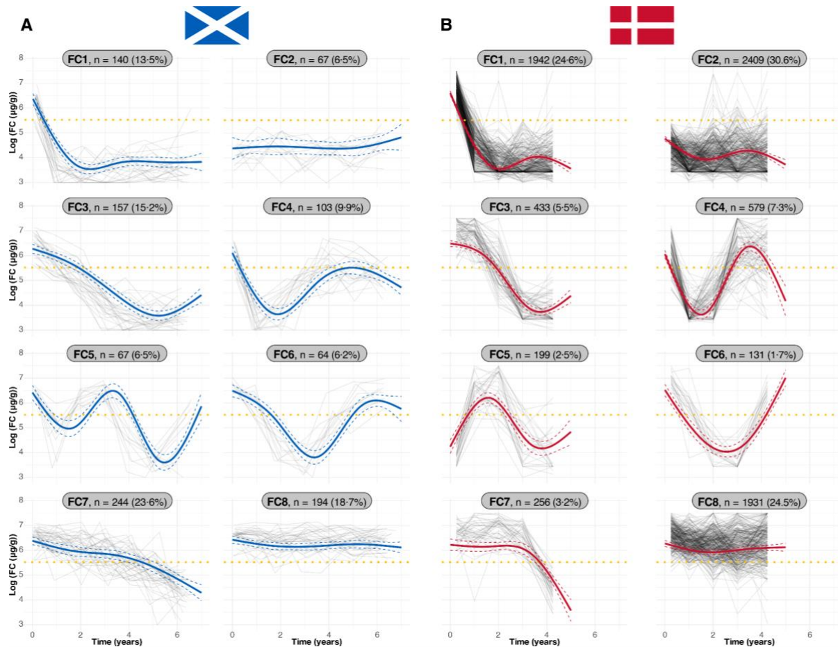
Figure 2. Cluster trajectories obtained from LCMM assuming eight clusters fitted to FC data (log-transformed) in (A) the Lothian IBD Registry and (B) Danish national registry data. The blue and red lines indicate predicted mean cluster profiles with 95% confidence intervals for the Lothian IBD Registry and Danish data respectively. The yellow dotted lines indicate \log(250\mu\text{g/g}) . For visualisation purposes, pseudo subject-specific trajectories have been generated by amalgamating observations from randomly selected groups of six subjects. Clusters are ordered from lowest (FC1) to highest (FC8) cumulative inflammatory burden in the Lothian data with Danish cluster labels chosen based on visual similarity to the former clusters. Cluster sizes are shown as panel titles.
