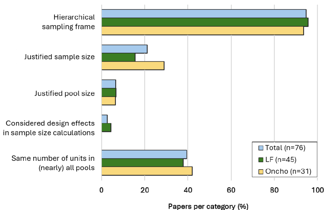
Fig. 3: Frequency of key design choices and justifications for the MX surveys in the included studies by disease and overall. Values are provided in Supplementary Table S2. Abbreviations LF: lymphatic filariasis; Oncho: onchocerciasis.
