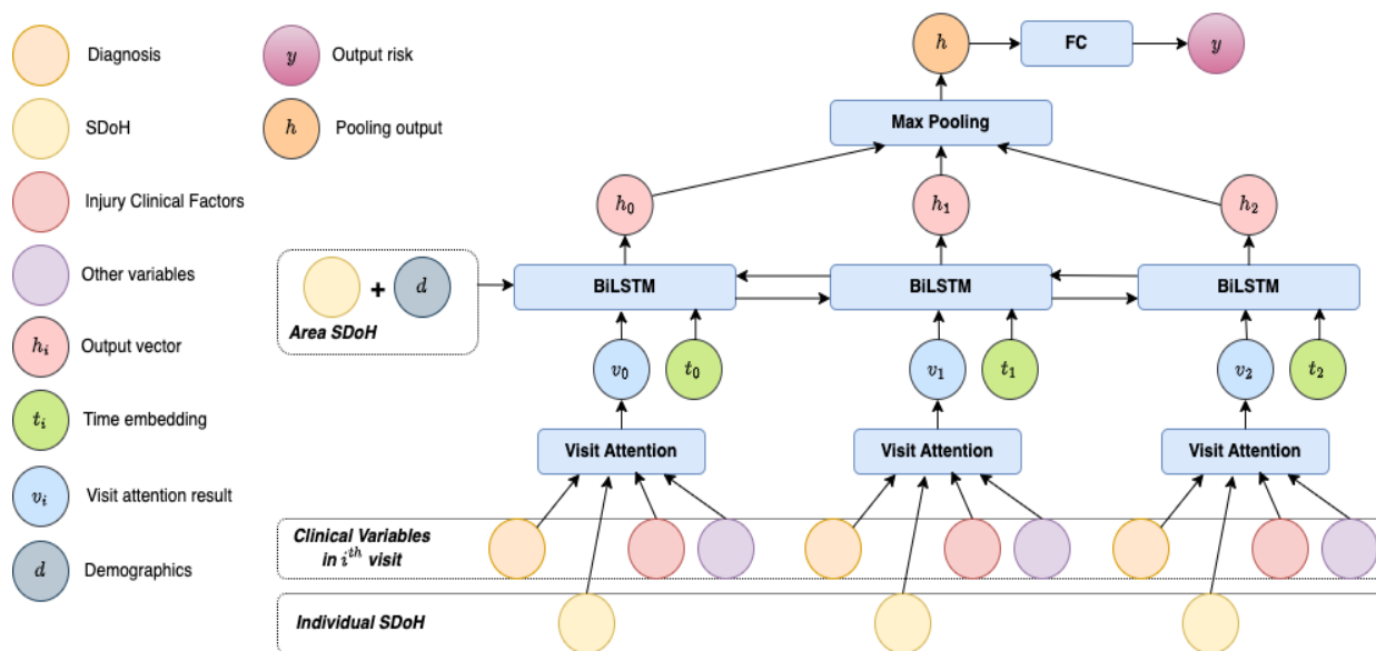
Figure 2. Illustration of our deep learning model based on a long short-term memory (LSTM) network.
