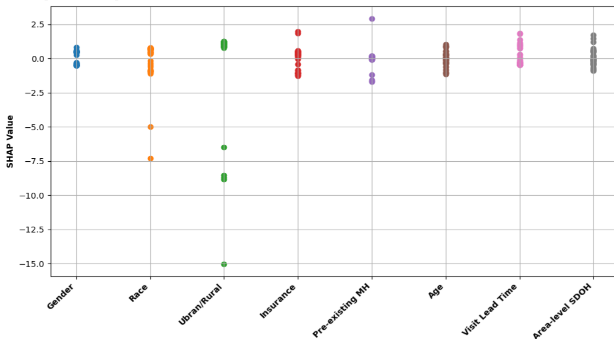
Figure 3. Illustration of Feature Contributions to BiLSTM Model Predictions Using SHAP Summary Plot. Visit Lead Time: number of days from index concussion diagnosis date to the first post-concussion visit date.
