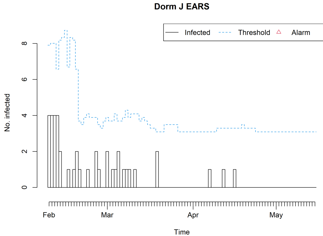
Figure 8: CDC EARS analysis of SARS-CoV-2 cases in Dorm J, 2021.
