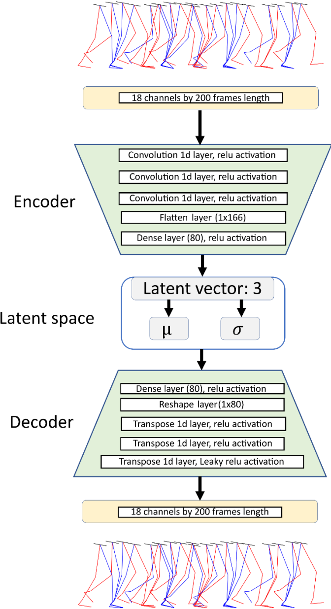
Figure S1: Network architecture of the variational autoencoder (VAE)
