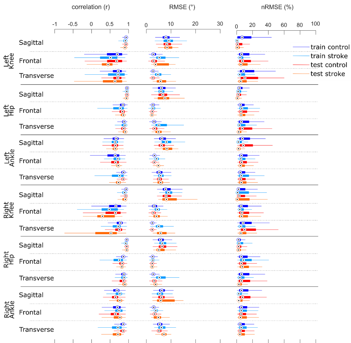
Figure S2: Validation results: Pearson's r , RMSE and nRMSE for all input channels. Red boxplots refer to the reconstruction accuracy of the test set. Blue boxplots refer to the reconstruction accuracy of the train set. Light blue and light red refer to the data of the stroke survivors, and dark blue and dark red represent the results of the healthy controls.
