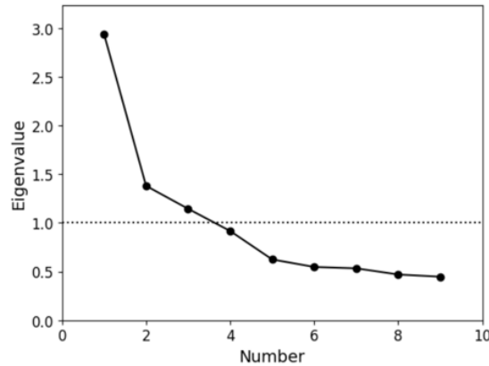
Scree Plot for Exploratory Factor Analysis of Original Nine-Item Survey in Study 1
