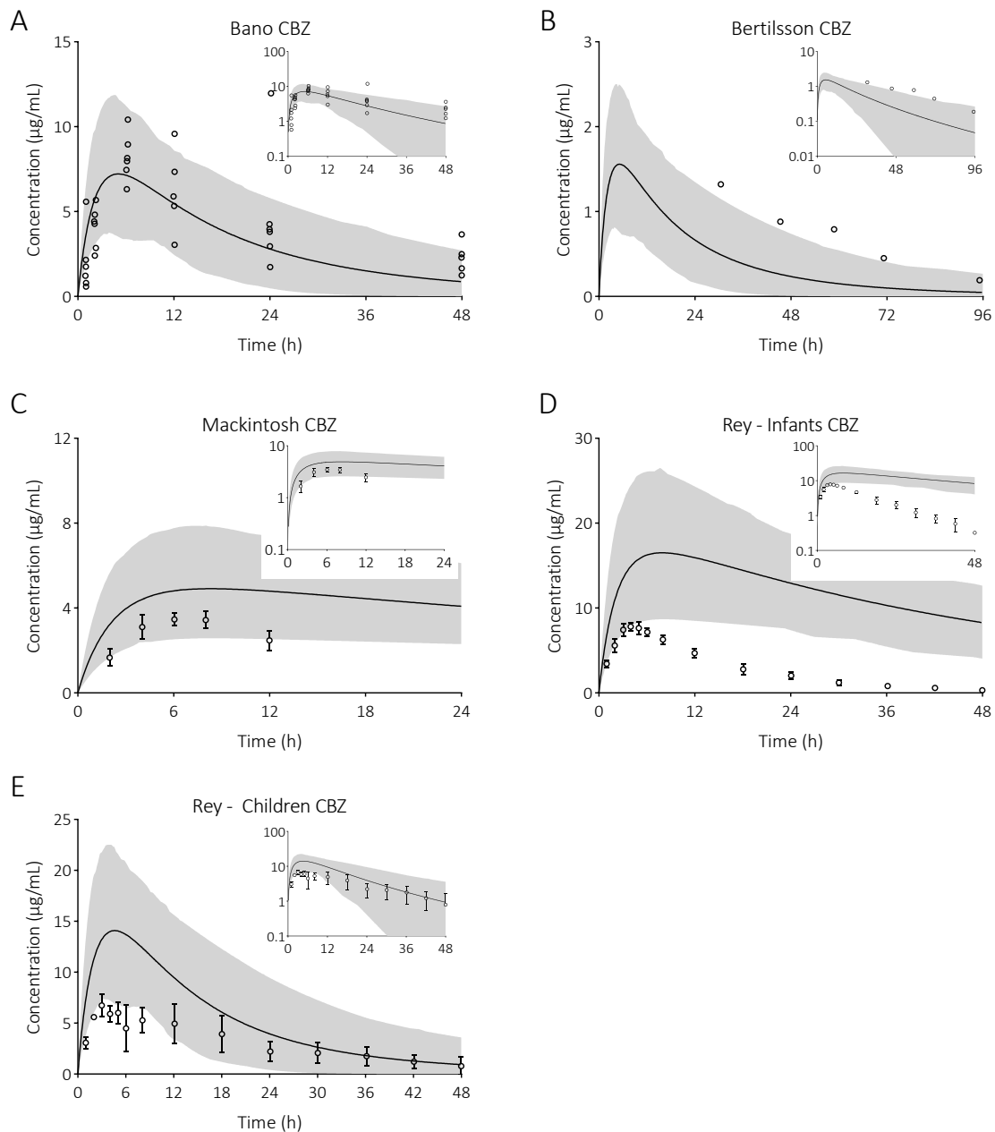
Figure 8. Prediction of carbamazepine (CBZ) and plasma concentration-time profiles in paediatric individuals upon single dose administration. The solid line is the predicted mean of the simulated population and the shaded area represents the 5 th to 95 th percentile of the virtual population. Open circles are the observed data: A (23), B (24), C (25), and D & E (26).
