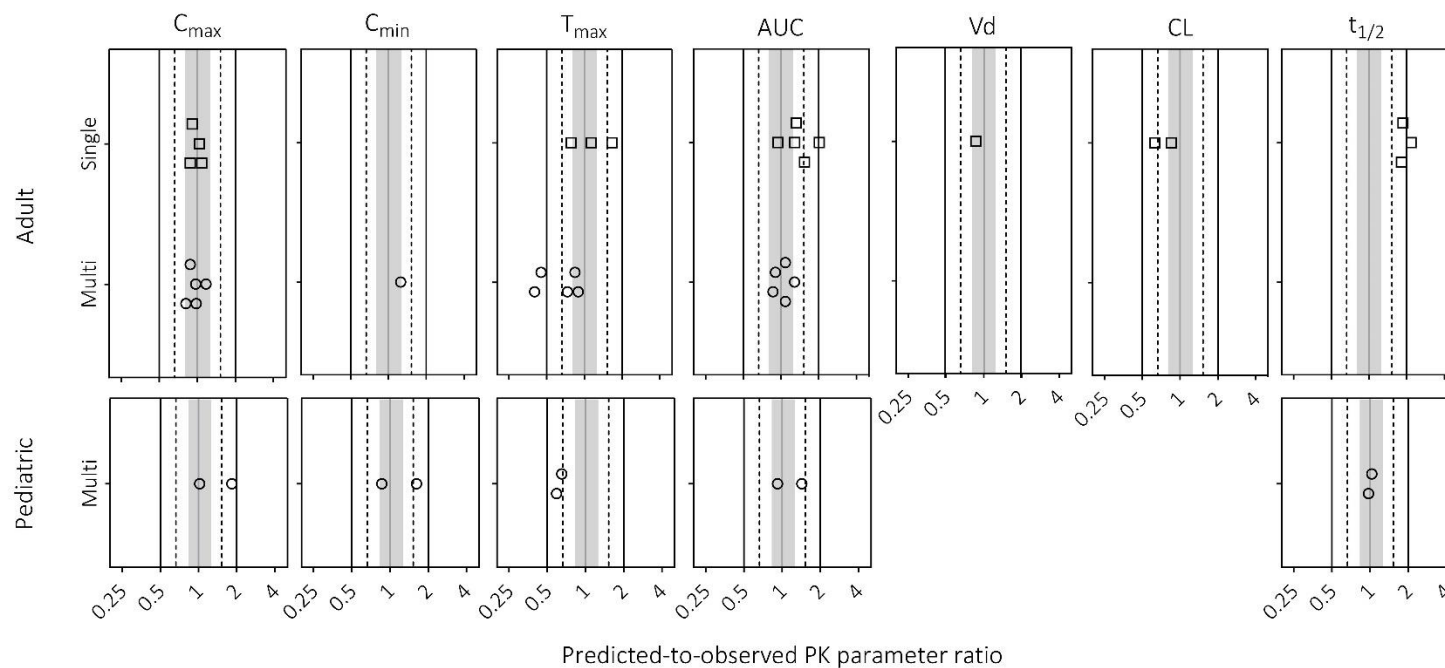
Figure 5. Predicted-to-observed ratios of the maximum concentration ( C_{max} ), minimum concentration ( C_{min} ), time to peak concentration ( T_{max} ), area under the curve (AUC), volume of distribution ( V_d ), clearance (CL), and half-life ( t_{1/2} ) for valproic acid extended-release formulations single- and multi-dose studies in adults and pediatrics. Single symbols represent a predicted-to-observed ratio of a single pharmacokinetic study. The black lines represent the 2-fold range, the dashed lines the 1.5-fold range, the gray shaded area represent the 1.25-fold range and the gray line represents the unity line.
