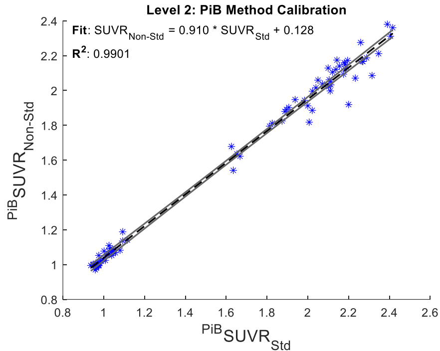
Figure S2 – Level 2 Centiloid calibration analysis for PiB using published Pittsburgh calibration data. The regression equation is substituted into the published Level 1 Centiloid equation to find:
