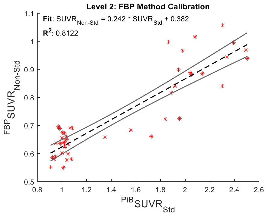
Figure S3 – Level 2 Centiloid calibration analysis for FBP using published Avid calibration data. The regression equation is substituted into the published Level 1 Centiloid equation to find:
