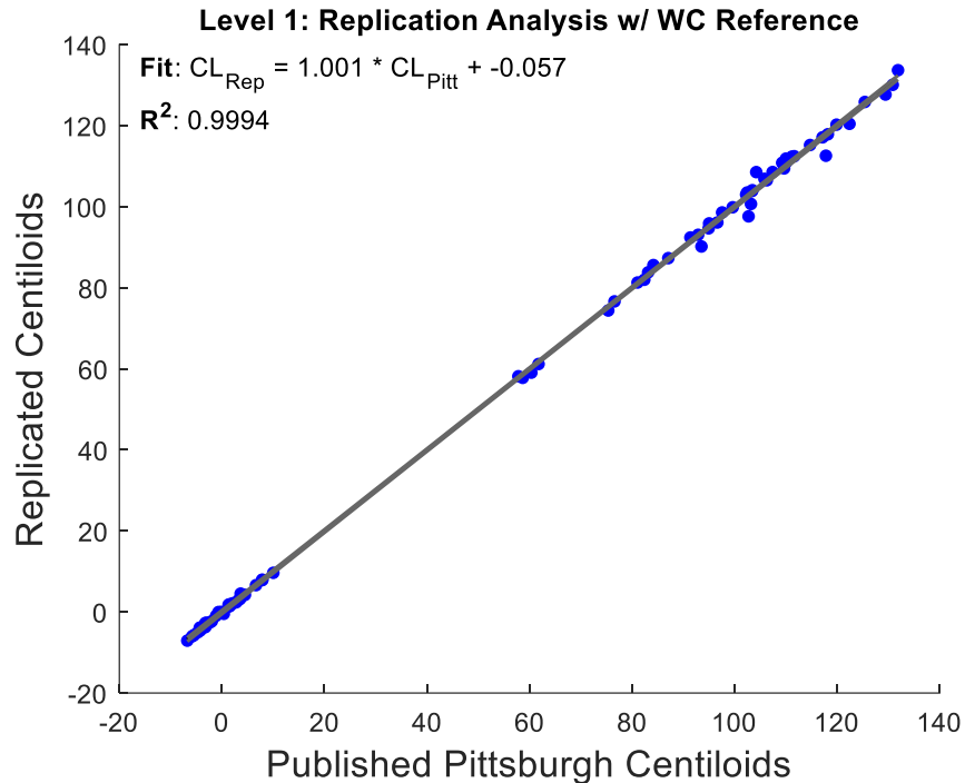
Figure S1 – Level 1 Centiloid replication analysis using published Pittsburgh calibration data.
