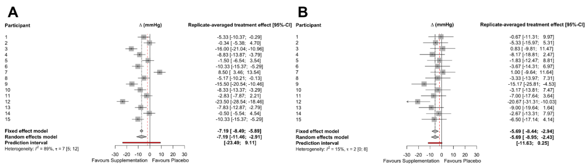
322 Figure 3. Forest plots for systolic BP (A) and diastolic BP (B) summary effects and between- 323 participant (t) replicated-averaged treatment effect heterogeneity. The red dashed line 324 indicates the target difference reduction of 2 mmHg. \tau , denotes tau-statistic; CI, denotes 325 confidence interval. 326
