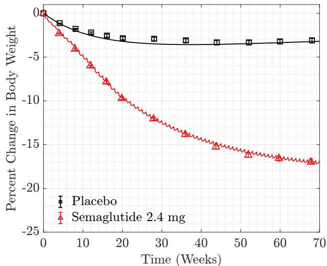
Figure S.1: Solid curves are the semaglutide PD model. Markers are clinical trial data from Wilding et al. [7].
