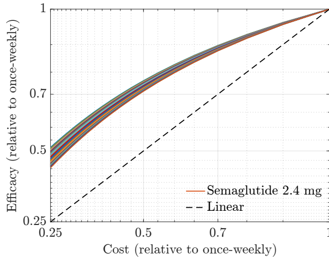
Figure S.2: Reducing cost by reducing dose frequency does not commensurately reduce weight loss efficacy for a wide range of values of the parameters E_{\max,\text{fast}} and E_{\max,\text{slow}} . See section S.1.3.1 for details.
