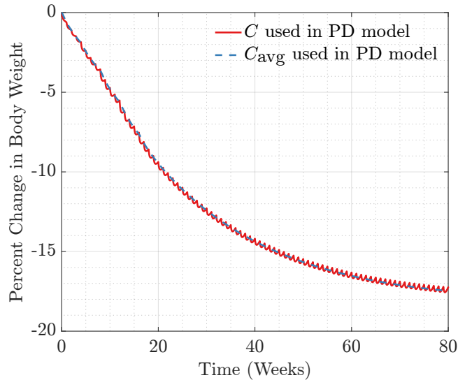
Figure S.3: Percent change in body weight over time for 2.4 mg once weekly dose of semaglutide. The curves are the semaglutide model in section S.1.3 using either the time-dependent semaglutide concentration C (red solid curve) or the weekly averaged semaglutide concentration C_{\text{avg}} (blue dashed curve).
