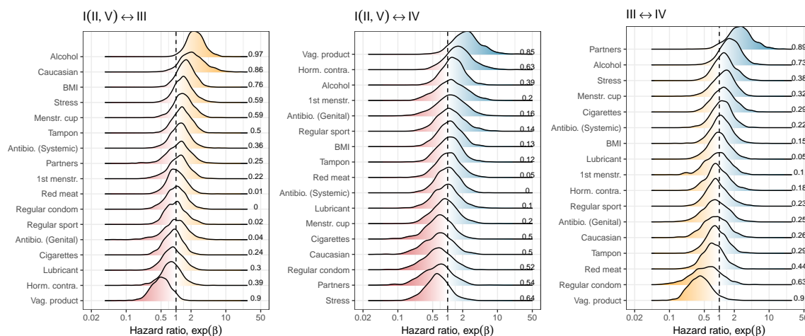
Figure 4: Estimated covariate effects on community transition rates. With the symmetry assumption, there are three sets of covariate effects on transitions. The impact of covariates on community transition rates was estimated for a given set of community states as the log hazard ratio, \beta . The figure shows the posterior distributions of \exp(\beta) , the hazard ratio for the three sets of transition sets, and the corresponding 16 covariates. The numbers on the right-hand side of each panel indicate the probability that the estimated effect is different from the hazard ratio of 1 (i.e., the proportion of posterior distributions sampled on the dominant side of the effect). For example, alcohol consumption was estimated to favour CST III over CST I (II,V) at a credibility level of 97%.
